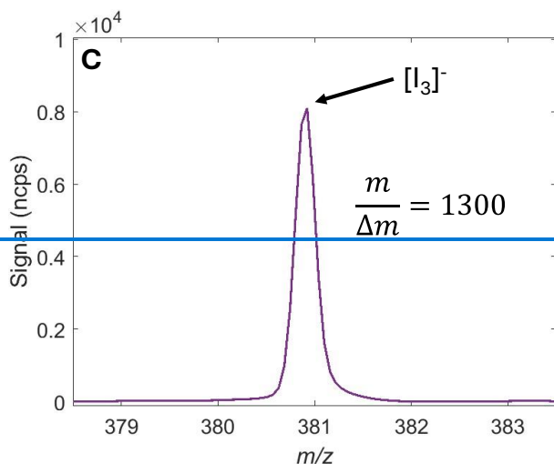
Figure 3: (a) Normalized high-resolution mass spectrum of a calibration gas over lab air in benzene cation mode with labelled analyte signals. (b) Normalized high-resolution mass spectrum of air measurements in the field in iodide anion mode with labelled analyte signals. (c) Zoom in on I_3^- cluster signal illustrating representative peak widths for the high-resolution mass spectrum in Fig. 3b.
