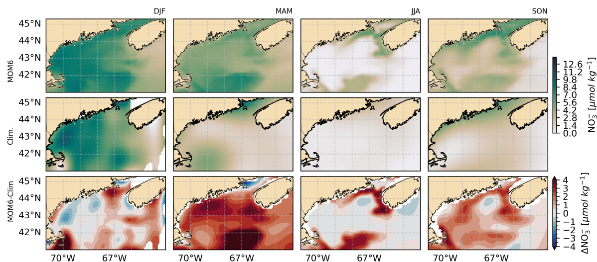
Figure 13. Seasonal surface distribution of nitrate in the Gulf of Maine region considering the climatology of surface concentrations from MOM6 (first row), a seasonal climatology calculated from Rebeck's dataset (second row), and their difference (MOM6 – Climatology). Columns represent seasons: DJF, MAM, JJA, SON.
