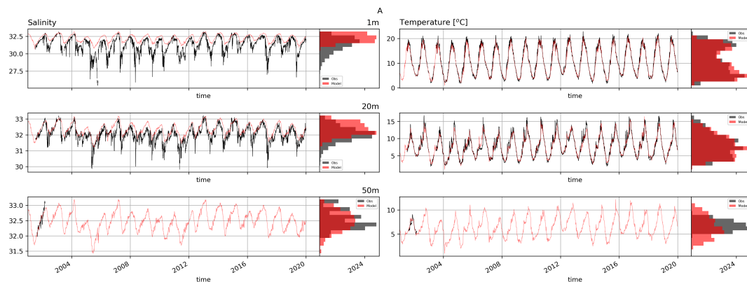
Figure A5. Time series of salinity in temperature of MOM6 (red) and NERACOOS mooring measurements (black) at buoy A01.
