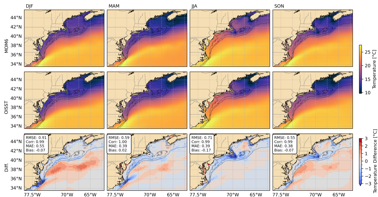
Figure 5. Seasonal averages of sea surface temperature considering MOM6 (top panels), OISST (middle panels) and their differences (lower panels, MOM6 - OISST). MOM6 results were upscaled to OISST resolution ( 0.25^\circ ) by binning corresponding areas and calculating averages. Black contours are the isobath of 40, 80, and 400 m.
