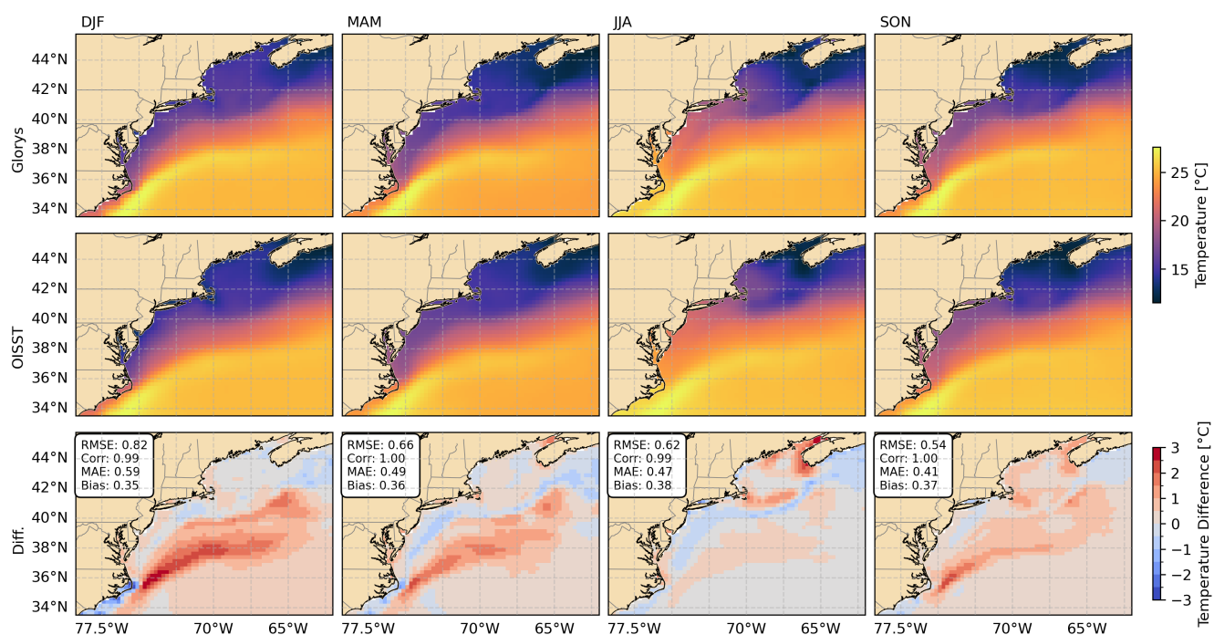
Figure A1. Seasonal averages of sea surface temperature considering Glorys (top panels), OISST (middle panels) and their differences (lower panels, Glorys - OISST). Glorys results were upscaled to OISST resolution ( 0.25^\circ ) by binning corresponding areas and calculating averages. Black contours are the isobath of 40, 80, and 400 m.
