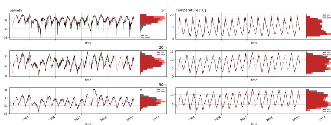
Figure A7. Time series of salinity in temperature of MOM6 (red) and NERACOOS mooring measurements (black) at buoy E01.
