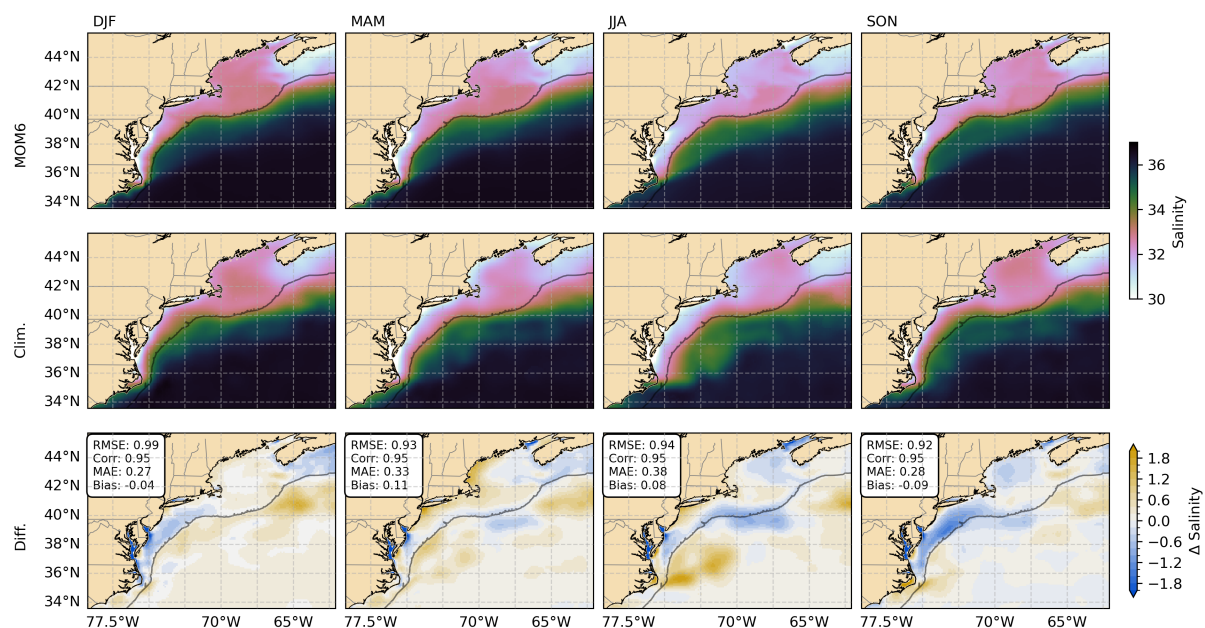
Figure 6. Seasonal averages of sea surface salinity from MOM6 (top panels) and NCEI regional climatologies (Clim., middle panels) and seasonal differences (lower panels, MOM6 - Clim.). Black contour indicates the 400m isobath, roughly representing the position of the shelf break. MOM6 results were upscaled to NCEI climatologies resolution ( 0.1^\circ ) by binning corresponding areas and calculating averages.
