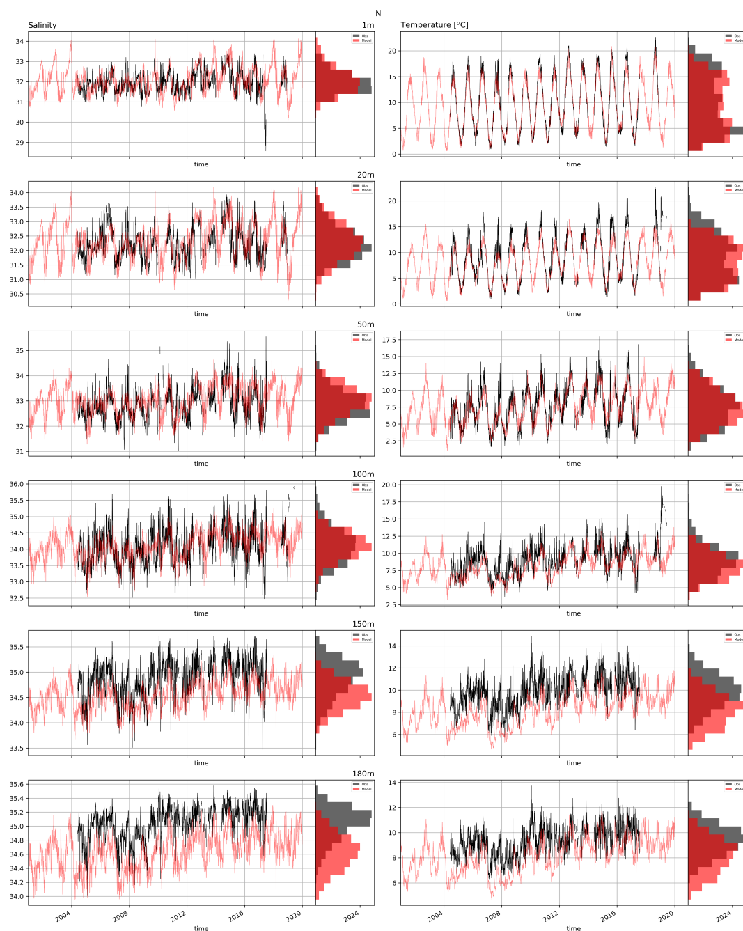
Figure A11. Time series of salinity in temperature of MOM6 (red) and NERACOOS mooring measurements (black) at buoy M01.
