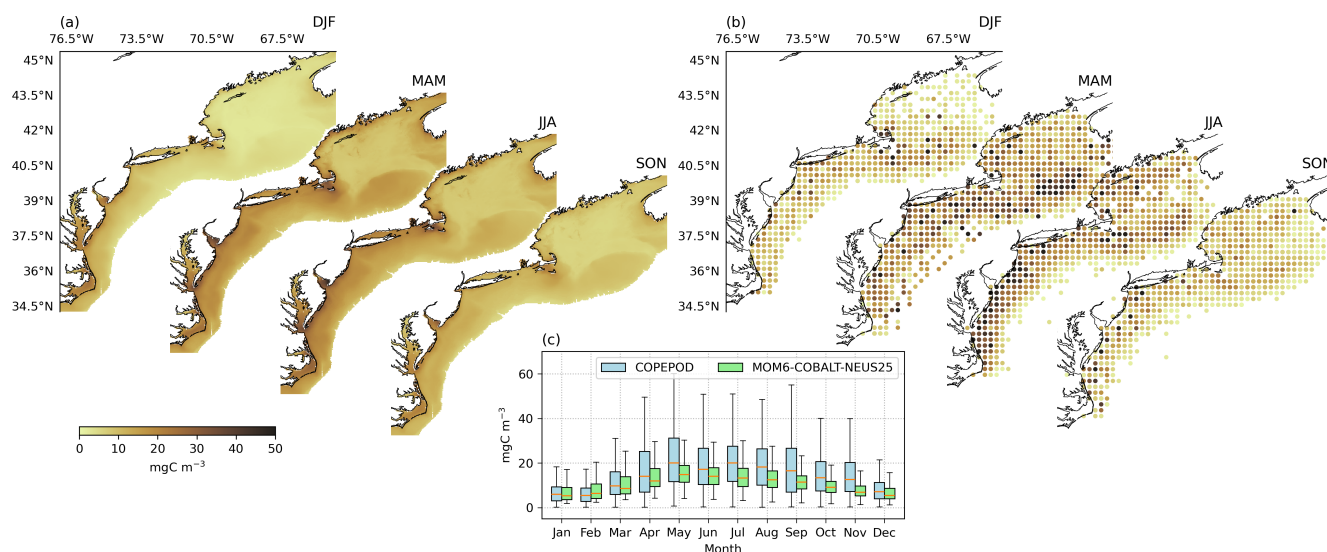
Figure 15. Seasonal averages carbon biomass (depth-averaged over the top 200 m) on the continental shelf (within the 400 m isobath) encompassing the Mid-Atlantic Bight, Georges Bank and Gulf of Maine for (a) MOM6-COBALT-NEUS25, and (b) COPEPOD dataset. Boxplots represent the distribution of the horizontal fields of monthly and depth-averaged biomass. Seasonal bias are (DJF, MAM, JJA, SON) (1.3, 5.7, 7.2, 10.9) \text{mgC m}^{-3} .
