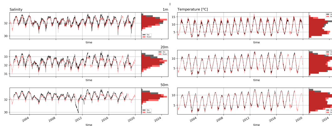
Figure A9. Time series of salinity in temperature of MOM6 (red) and NERACOOS mooring measurements (black) at buoy I01.
