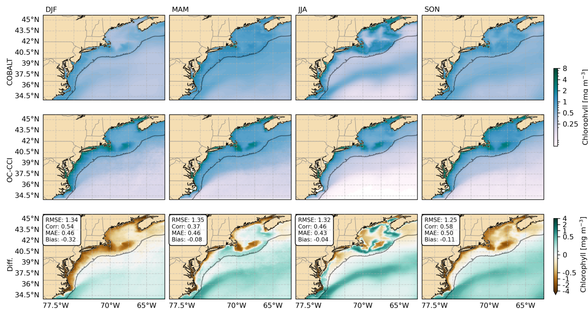
Figure 14. Difference between seasonal averages of surface chlorophyll from MOM6-COBALT-NEUS25 results and OC-CCI satellite data product.
