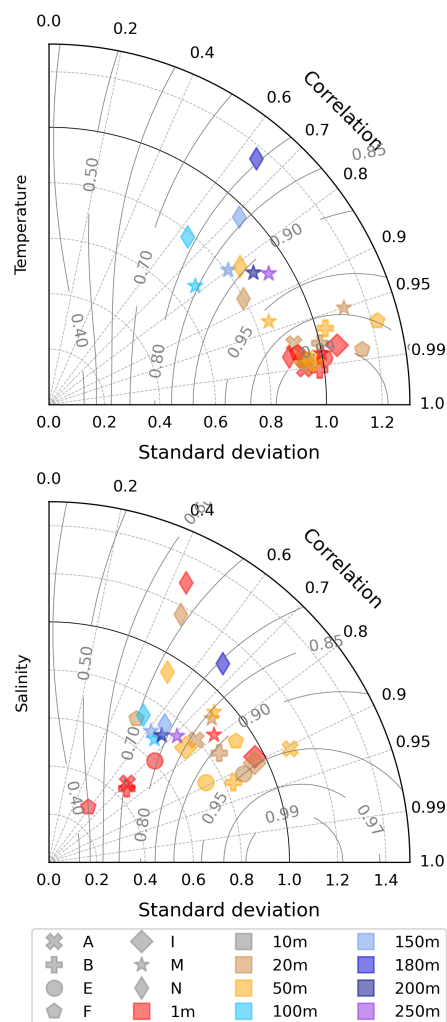
Figure 10. Taylor diagram evaluating MOM6 (upper panel) daily temperature and (lower panel) salinity performance against NERACOOS measurements. Gray shapes in the legend represent the mooring identification, while colors represent measurement depths. The standard deviation of the model results is normalized by the standard deviation of the observations. Curved contours represent isolines of skill score (Willmott, 1981).
