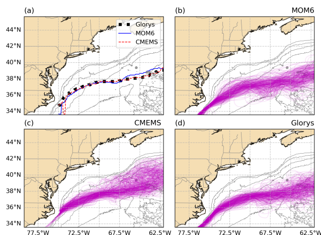
Figure 2. Path comparison of the Gulf Stream for the period between the years of 1993-1994 across MOM6, CMEMS satellite SSH L4 product and Glorys. The position of the Gulf Stream based on the maximum standard deviation of SSH is presented in the upper left panel. In the remaining panels, magenta lines represent the 0 m contour of monthly SSH anomaly.
