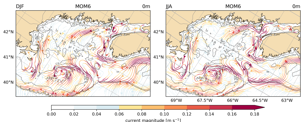
Figure 3. Streamlines of MOM6 surface currents in winter (DJF) and summer (JJA) in the Gulf of Maine.
