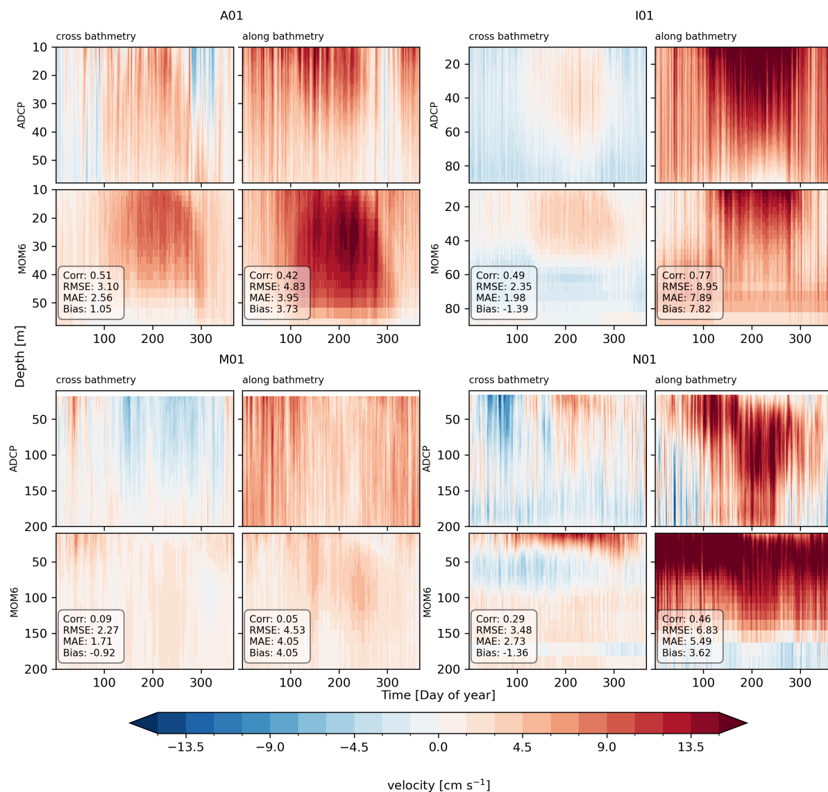
Figure 4. Hovmöller diagram of currents (daily composite) measured by NERACOOS ADCP and simulated by MOM6-COBALT-NEUS25 (row labels), considering cross-, and along-bathymetry currents. Positive values of along-bathymetry panels are referenced as equatorward flow for moorings A01, and I01, towards the Gulf of Maine at N01, and in the cyclonic direction at M01. In the cross bathymetric panels, positive values are perpendicular and to the right of the along-bathymetry direction. The evaluation period spans the years between 2009 to 2019 and correlation values represent the correlation between observed and modeled currents computed over all time-depth pairs (flattened time-depth matrix). The position of the moorings is found in Figure 1
