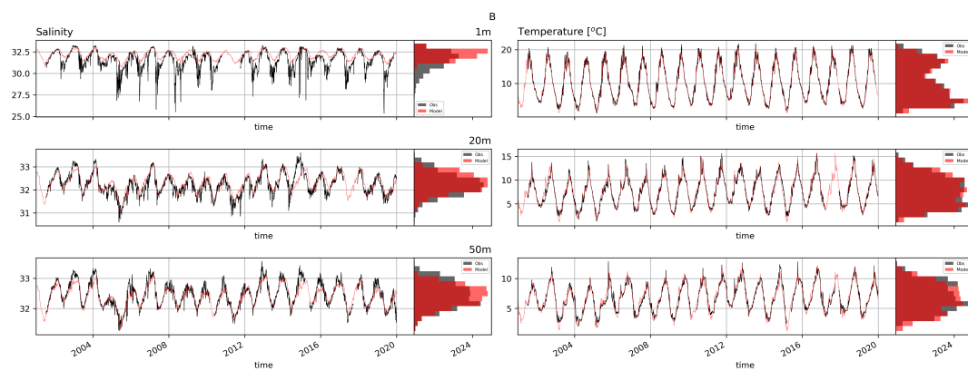
Figure A6. Time series of salinity in temperature of MOM6 (red) and NERACOOS mooring measurements (black) at buoy B01.
