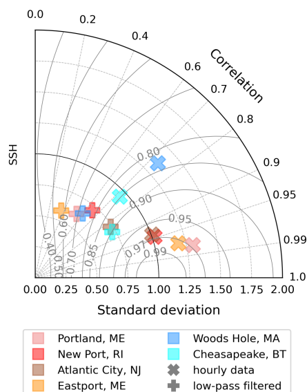
Figure 12. Taylor diagram of hourly SSH data at tide gauges at multiple coastal areas in the Gulf of Maine and Mid-Atlantic Bight alongside low-pass data with a cutoff period of 24 hours (Lanczos filter). The standard deviation of the model results is normalized by the standard deviation of the observations. Curved contours represent isolines of skill score (Willmott, 1981).
