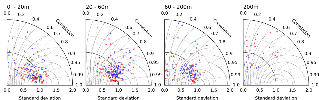
Figure A4. Taylor Diagrams of bottom temperature measurements in lobster thermistors at different bathymetry intervals considering MOM6 (red) and Glorys (blue) results.
