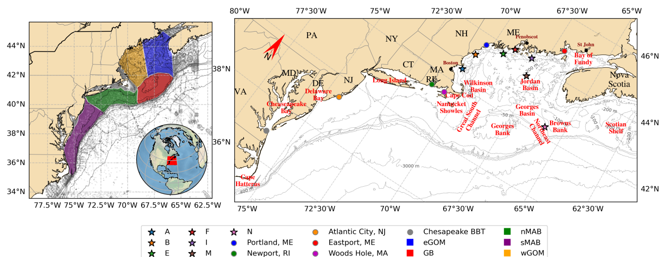
Figure 1. Model domain, Bathymetry, Observations (left panel), and locations references (right panel): Stars represent NERACOOS moorings, circles indicate CO-OPS tide gauges, and grey dots show high-resolution CTD data from the World Ocean Database. Colored shapes mark the locations of eastern Gulf of Maine (eGOM), western Gulf of Maine (wGOM), Georges Bank (GB), northern Mid-Atlantic Bight (nMAB), and southern Mid-Atlantic Bight (sMAB).
