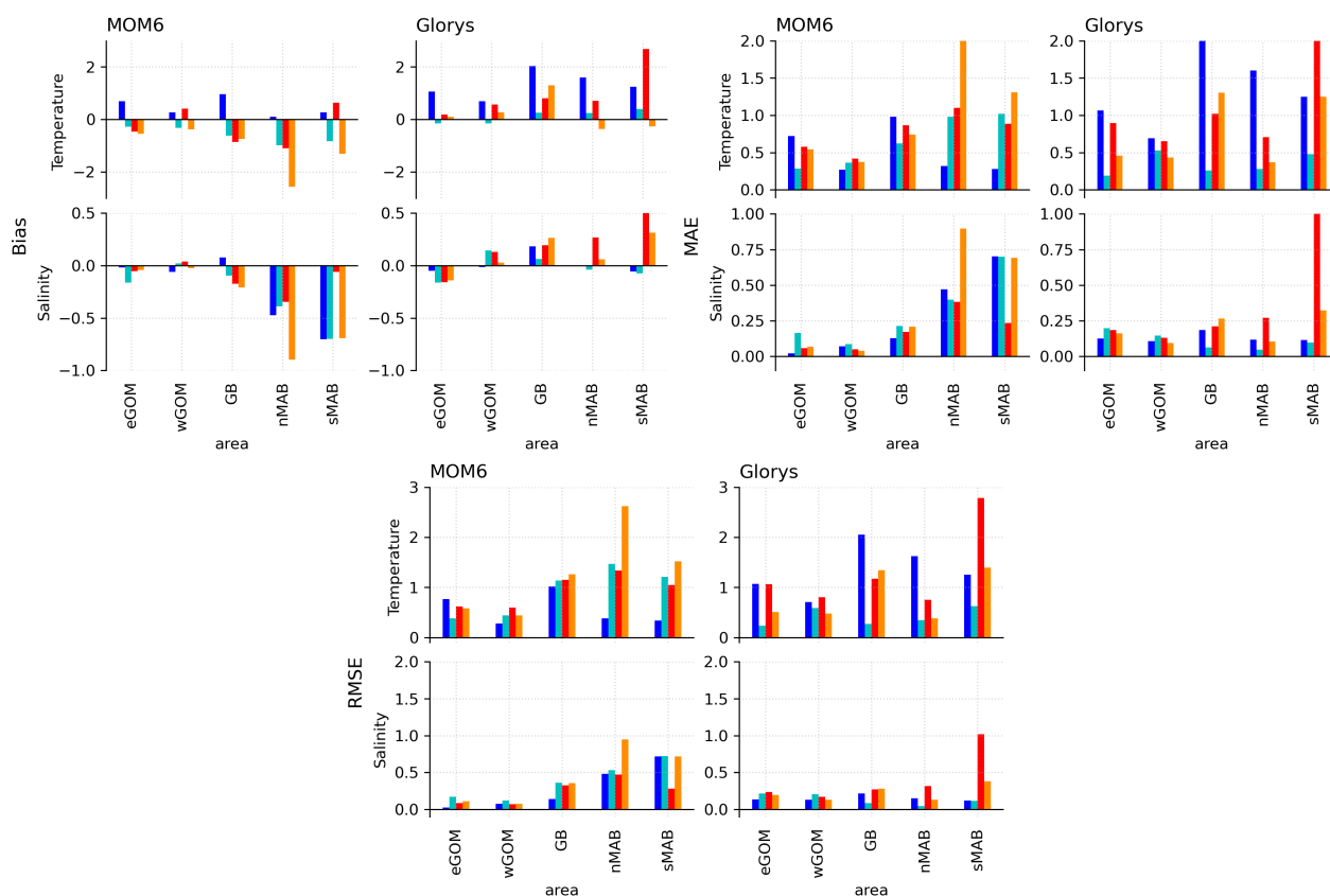
Figure A3. Error statistics of seasonal average profiles at different subdomains of the model. Colors represent winter (blue), spring (cyan), summer (red), and fall (orange)
