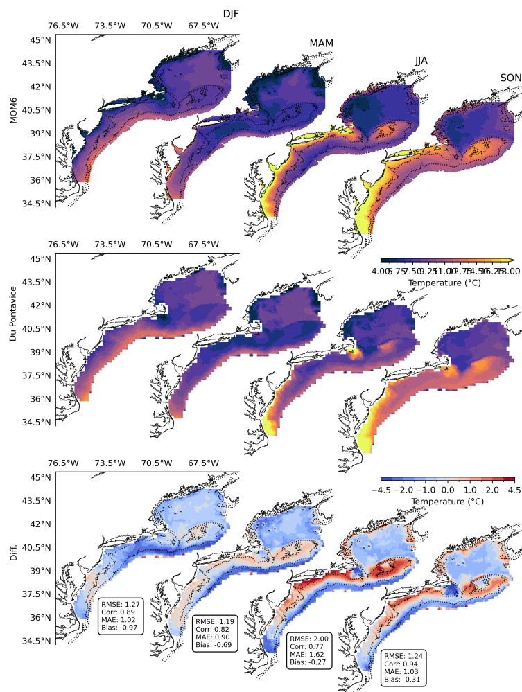
Figure 7. Seasonal averages of bottom temperature in MOM6 (upper panels), Du Pontavice bottom temperature dataset (mid panels), and their difference (MOM6 - duPontavice) considering the period between 1993 to 2019. Dotted lines correspond to the isobaths of 40 and 80 m. MOM6 results were upscaled to Du Pontavice's resolution ( 1/12^\circ ) by binning corresponding areas and calculating averages.
