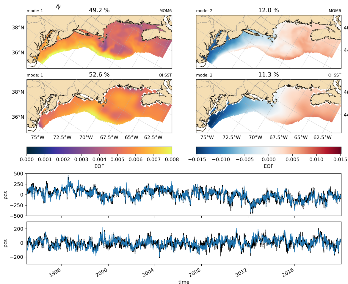
Figure 11. First (left panels) and second (right panels) modes of empirical orthogonal functions and principal component time series considering SST daily anomalies of MOM6 (top panels) and OISST (bottom panels). For the first (second) mode of principal components correlation, normalized standard deviation, mean bias and absolute error are 0.93, 0.99, -3.57, and 35 (0.78, 0.93, -0.38, 29), respectively. The explained variance of MOM6 (OI SST) first mode is 49.5 % (52.7 %), while the second mode has 12.1% (11.5 %)
