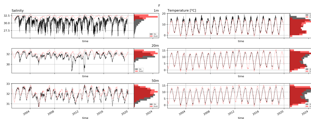
Figure A8. Time series of salinity in temperature of MOM6 (red) and NERACOOS mooring measurements (black) at buoy F01.
