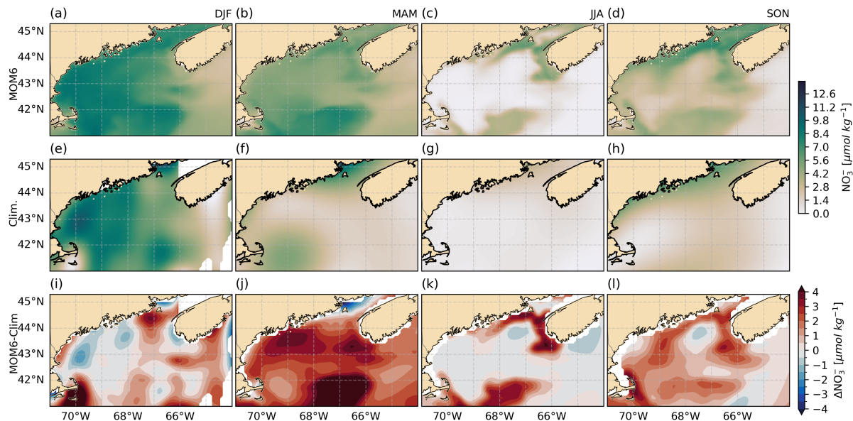
Figure 14. Seasonal surface distribution of nitrate in the Gulf of Maine region considering the climatology of surface concentrations from MOM6 (a to d), a seasonal climatology calculated from Rebeck's dataset (e to h), and their difference (i to l) (MOM6 – Climatology). Columns represent seasons: DJF, MAM, JJA, SON.
