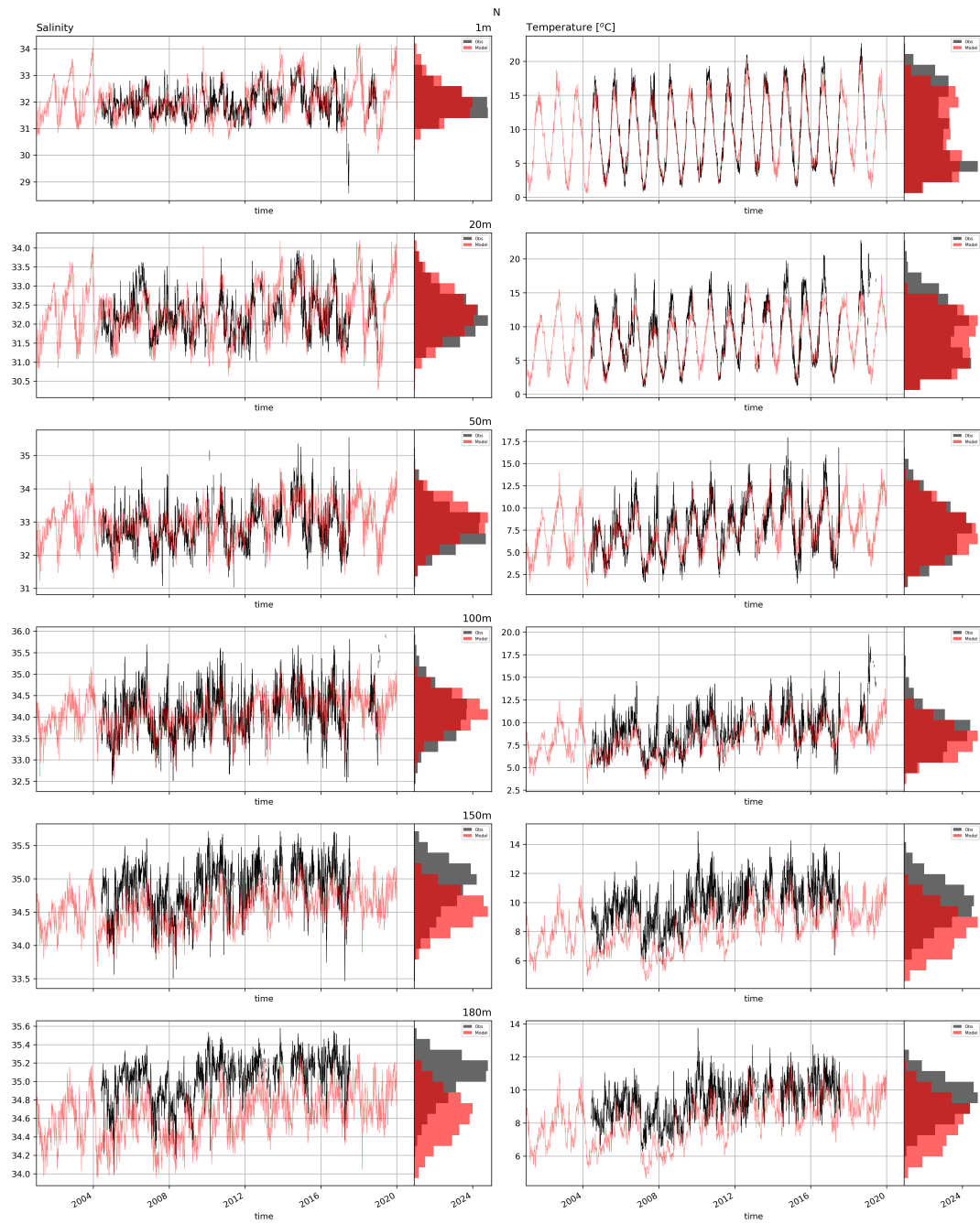
Figure A12. Time series of salinity in temperature of MOM6 (red) and NERACOOS mooring measurements (black) at buoy M.
