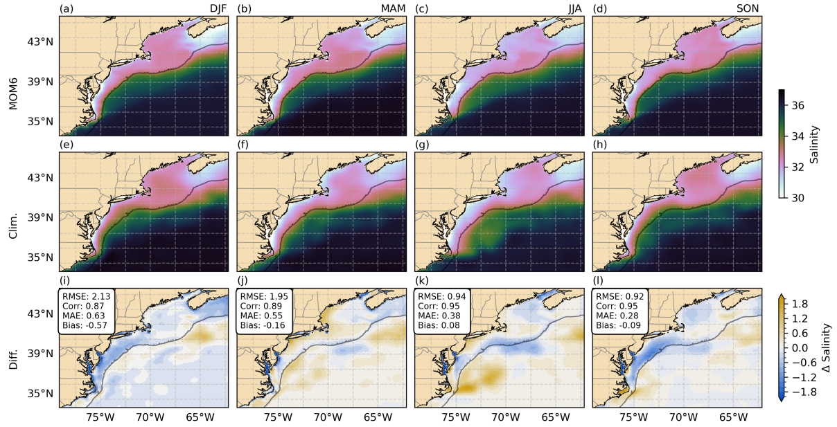
Figure 7. Seasonal averages of sea surface salinity from MOM6 (a to d) and NCEI regional climatologies (Clim., e to h) and seasonal differences (MOM6 - Clim., i to l). Black contour indicates the 400m isobath, roughly representing the position of the shelf break. MOM6 results were upscaled to NCEI climatologies resolution ( 0.1^\circ ) by binning corresponding areas and calculating averages.
