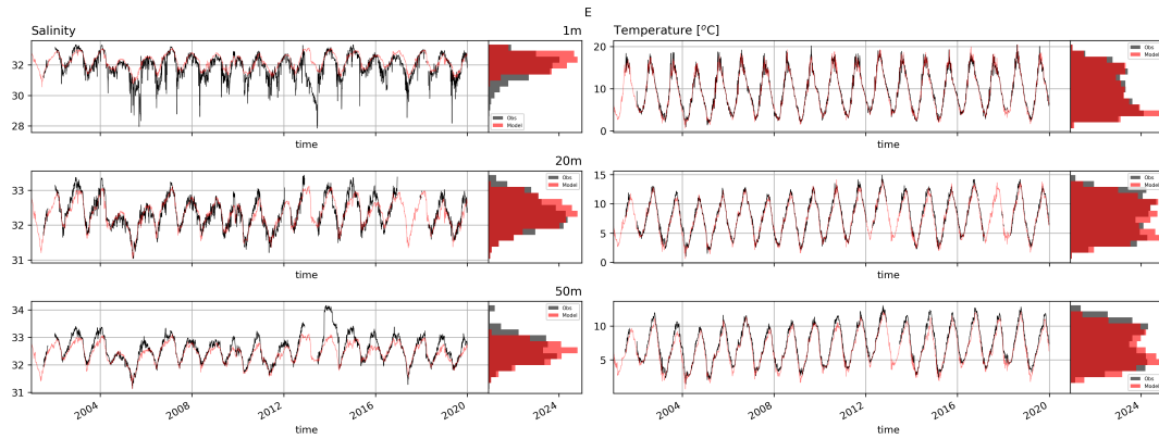
Figure A8. Time series of salinity in temperature of MOM6 (red) and NERACOOS mooring measurements (black) at buoy E.
