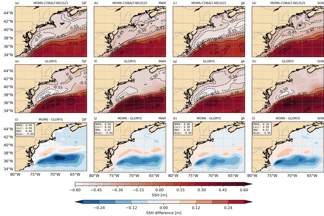
Figure 3. Seasonal averages of SSH considering MOM6-COBALT-NEUS25 (a to d), GLORYS (e to h) and their difference, MOM6-COBALT-NEUS25 - GLORYS (i to l). Black contours and filled contours represent SSH intervals.
