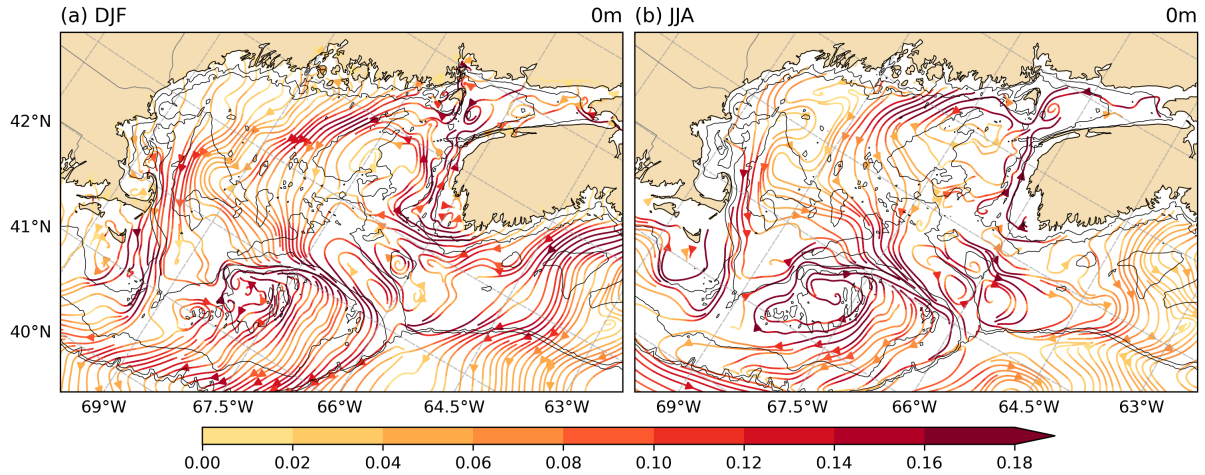
Figure 4. Winter (a) and summer (b) integral curves of the instantaneous MOM6 surface velocity field, computed via numerical integration of the tangent vector field.
