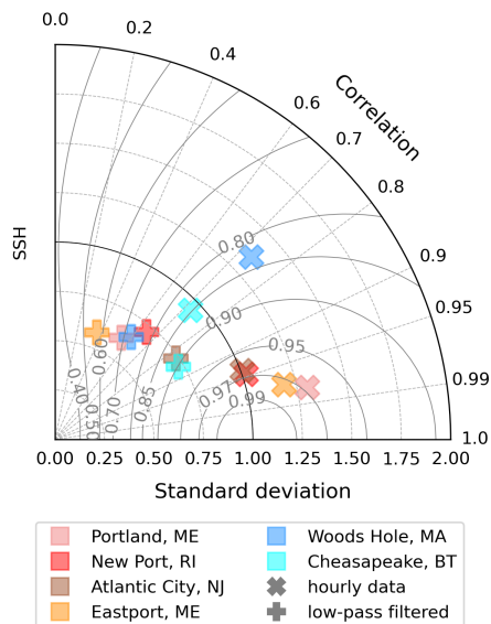
Figure 13. Taylor diagram of hourly SSH data at tide gauges at multiple coastal areas in the Gulf of Maine and Mid-Atlantic Bight alongside low-pass data with a cutoff period of 24 hours (Lanczos filter). The standard deviation of the model results is normalized by the standard deviation of the observations. Curved contours represent isolines of skill score (Willmott, 1981).
