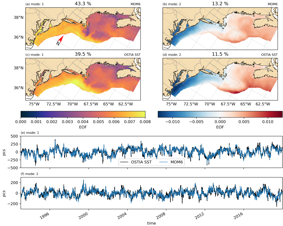
Figure 12. First (a,c,e) and second (b,d,f) modes of empirical orthogonal functions and principal component time series considering SST detrended daily anomalies of MOM6 (a,b) and OSTIA SST (c,d). For the first (second) mode of principal components correlation, normalized standard deviation, mean bias and mean absolute error are 0.94, 1.04, 0.4487, and 167.73 (0.88, 1.02, -0.08, 27.74), respectively. The explained variance of MOM6 (OSTIA SST) first mode is 43.3 % (39.5 %), while the second mode has 13.2% (11.5%).
