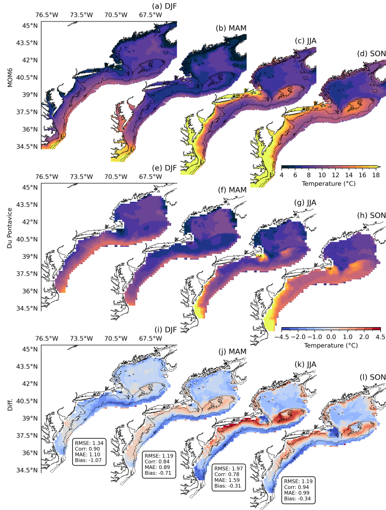
Figure 8. Seasonal averages of bottom temperature in MOM6 (a to d), Du Pontavice bottom temperature dataset (e to h), and their difference (MOM6 - duPontavice, i to l) considering the period between 1993 to 2019. Dotted lines correspond to the isobaths of 40 and 80 m. MOM6 results were upscaled to Du Pontavice's resolution ( 1/12^\circ ) by binning corresponding areas and calculating averages.
