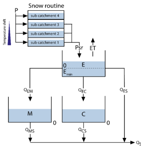
Fig. 3: Structure of the KarstMod rainfall-snow-discharge model designed for the Dévoluy case study. Snow routine converts rain into snow and vice versa, and gives input liquid precipitation ( P_{sr} ). E, M and C are compartments for flow transfer to the Spring (S). Q_{ES} is a direct flow from E to the spring.
