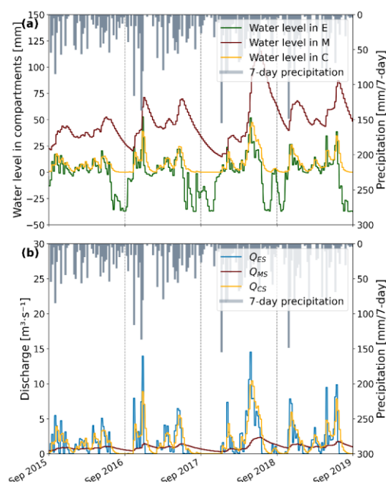
Fig. 5-7: (a) Model 2-Median of 5,000 simulations of seven-day averaged simulated water levels of KarstMod in compartments E, M, and C. (b) Median of 5,000 simulations of seven-day averaged internal KarstMod discharges (QES: discharge from E to S, QMS: discharge from M to S, QCS: discharge from C to S). Seven-day cumulative precipitation is shown on a secondary y-axis (inverted).
