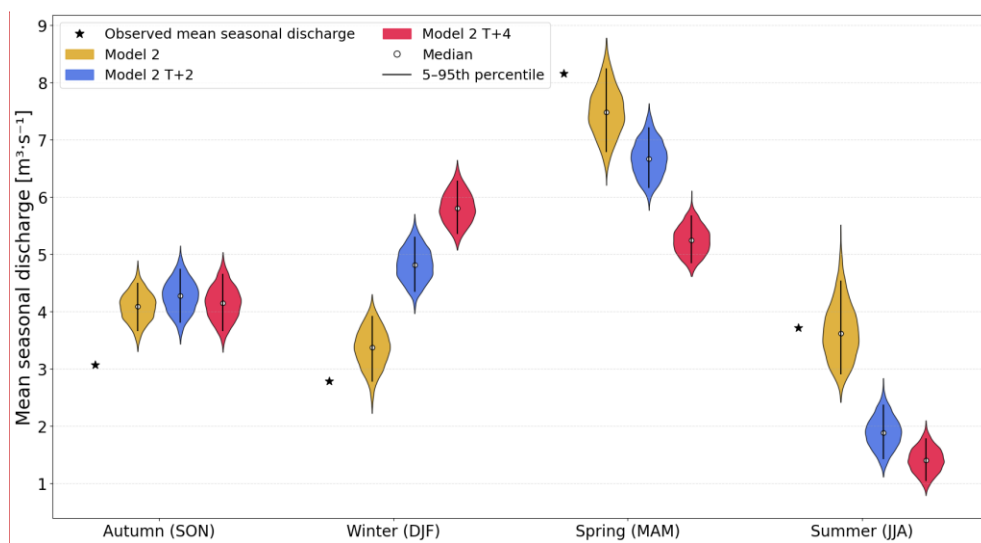
Fig. 9: Mean seasonal discharge distributions for the Dévoluy karst system over the 2015-2019 period according to scenario simulation described in Fig. 4. For each season, the star symbol indicates the observed mean seasonal discharge. Violin plots show the distribution of mean seasonal discharge across the 5,000 parameter set for Model 2 (gold), Model 2 T+2°C (blue), and Model 2 T+4°C (red). The vertical bar and white dot indicate the 5th-95th percentile range and the median of the 5,000 parameter set.
