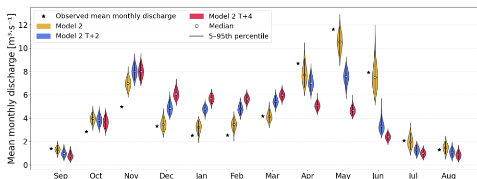
Fig. 10: Mean monthly discharge distributions for the Dévoluy karst system over the 2015-2019 period, shown for each calendar month (September to August) according to scenario simulation described in Fig. 4. For each month, the star symbol indicates the observed mean monthly discharge. Violin plots show the distribution of mean monthly discharge across the 5,000 parameter set for Model 2 (gold), Model 2 T+2°C (blue), and Model 2 T+4°C (red). The vertical bar and white dot indicate the 5-95th percentile range and the median of the 5,000 parameter set.
