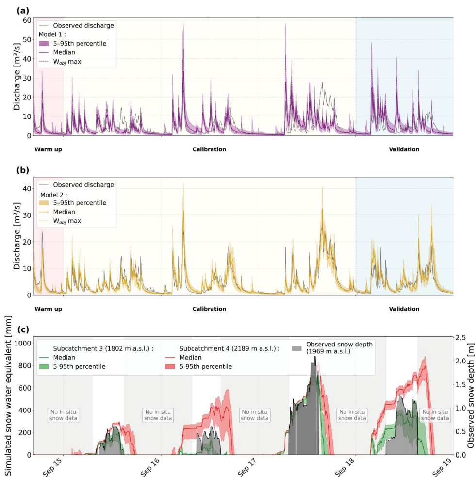
Fig. 4. Simulated and observed discharge of the Gillardes Spring compared to the observed discharge, between May for the Dévoluy karst system (2015 to September 2019) for (a) with Model 1 (without and (b) Model 2. Shaded areas show the 5th-95th percentile of the 5000-parameter set, solid lines the ensemble median, and dashed lines the W_{obj\ max} simulation. (c) Model 2 simulated snow routine), (b) Model 2 (with snow routine) and (c) snow comparison between in situ water equivalent for subcatchments 3 and 4 (shaded: 5th-95th percentile) and observed snow depth at the Super-Dévoluy ski resort versus simulated water stored in snowpack in the sub-catchments of the snow routine station (grey bars); gaps indicate periods with no available measurements.
