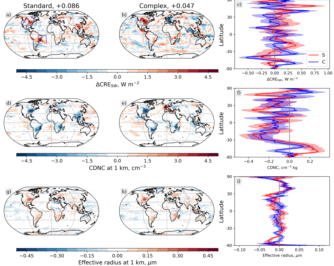
Figure 5. The role of the cloud radiative effect (CRE) in pre-industrial to present-day land use forcing. Subplots a-c show changes in the top of atmosphere fluxes from \Delta CRE_{SW} associated with land cover changes for the standard (s, left column) and complex (c, middle column) chemistry mechanism, as well as the zonal mean \Delta CRE_{SW} values for both mechanisms (right column). The changes in cloud droplet number concentrations (CDNC) at 1km altitude are displayed in subplots d), e) and f), while subplots g), h) and i) show the differences in effective radius at 1km altitude. Stippling in the left and middle columns shows regions of significant differences based on Student's t-test with 95% confidence, while shading on the zonal plots shows the standard error. The purple boxes on subplot a) mark regions of more substantial \Delta CRE_{SW} impacts that have been studied in additional detail.
