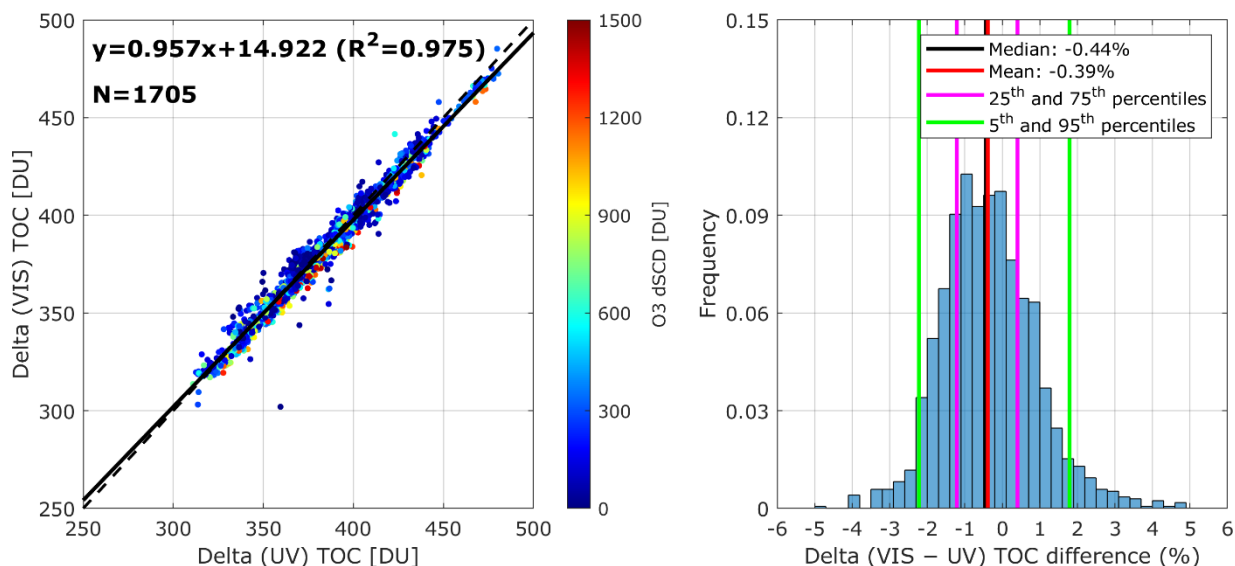
515 Figure 6: Comparison of TOC measurements from the UV and VIS channels of Delta over the study period. (left) Scatter plot of VIS against UV retrievals, color-coded by ozone dSCDs. The dashed line represents the 1:1 reference, while the solid line shows the linear regression fit. N corresponds to the total number of Delta measurements. (right) Frequency distribution of their respective percentage differences (VIS – UV). The vertical lines indicate the median (black), mean (red), the 25 th and 75 th percentiles (magenta), and the 5 th and 95 th percentiles (green).
