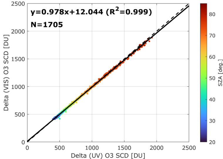
485 Figure 5: Comparison of ozone SCDs retrieved from Delta UV and VIS spectra over the study period. The data are color-coded by SZA. The dashed line represents the 1:1 reference, while the solid line shows the linear regression fit. N corresponds to the total number of Delta measurements.
