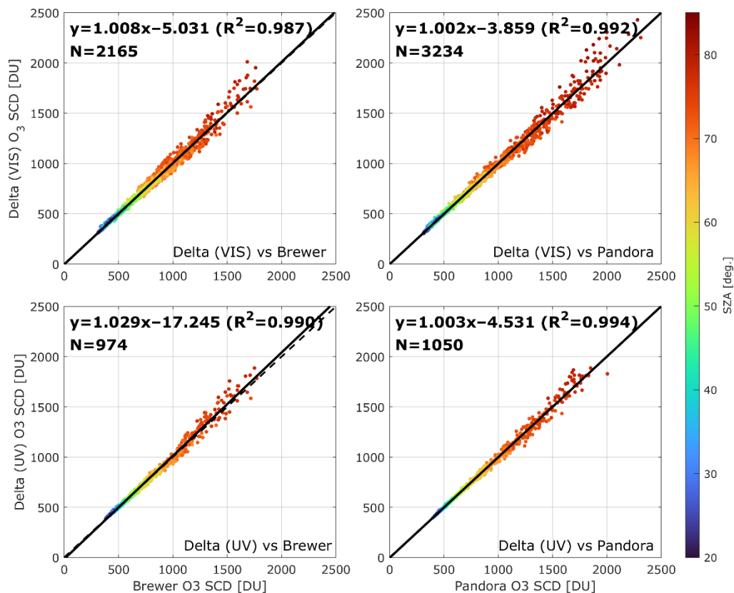
560 Figure 7: Intercomparison of ozone SCDs retrieved by Delta against the Brewer and Pandora instruments. Top row: Delta VIS compared to the Brewer (left) and the Pandora (right). Bottom row: Delta UV compared to the Brewer (left) and the Pandora (right). Data points are color-coded by SZA. The dashed lines indicate the 1:1 reference, while the solid lines show the fitted regression. N corresponds to the number of collocated measurements.
