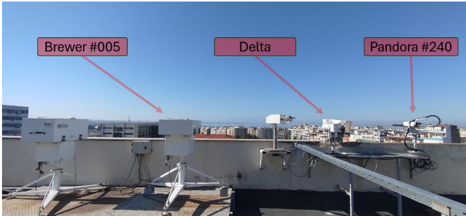
Figure 1: The measurement site of LAP.AUTH and the three collocated ground-based instruments used in this study: Brewer spectrophotometer #005 (left), Delta UV-VIS DOAS system (centre), and Pandora #240 (right).
