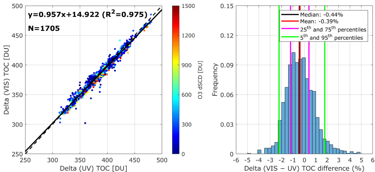
525 Figure 6: Comparison of TOC measurements from the UV and VIS channels of Delta over the study period. (left) Scatter plot of VIS against UV retrievals, color-coded by ozone dSCDs. The dashed line represents the 1:1 reference, while the solid line shows the linear regression fit. N corresponds to the total number of Delta measurements. (right) Frequency distribution of their respective percentage differences (VIS – UV). The vertical lines indicate the median (black), mean (red), the 25 th and 75 th percentiles (magenta), and the 5 th and 95 th percentiles (green).
