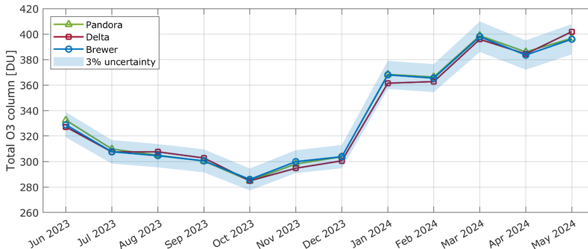
675 Figure 12: The seasonal variability of TOC captured by Pandora (green), Delta VIS (red), and Brewer (blue). The shaded blue area represents the \pm 3\% uncertainty range around the Brewer observations.
