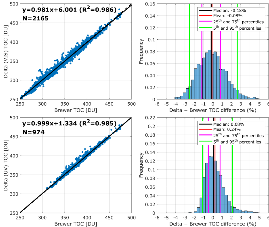
585 Figure 8: Comparison of TOC measurements from Delta and the Brewer. The left panels show scatter plots of collocated TOC retrievals from Delta VIS (top) and Delta UV (bottom), with regression fits (solid line) and the 1:1 reference (dashed line). N corresponds to the number of collocated measurements. The right panels show the corresponding frequency distributions of TOC percentage differences (Delta–Brewer), with mean, median, and percentile ranges indicated.
