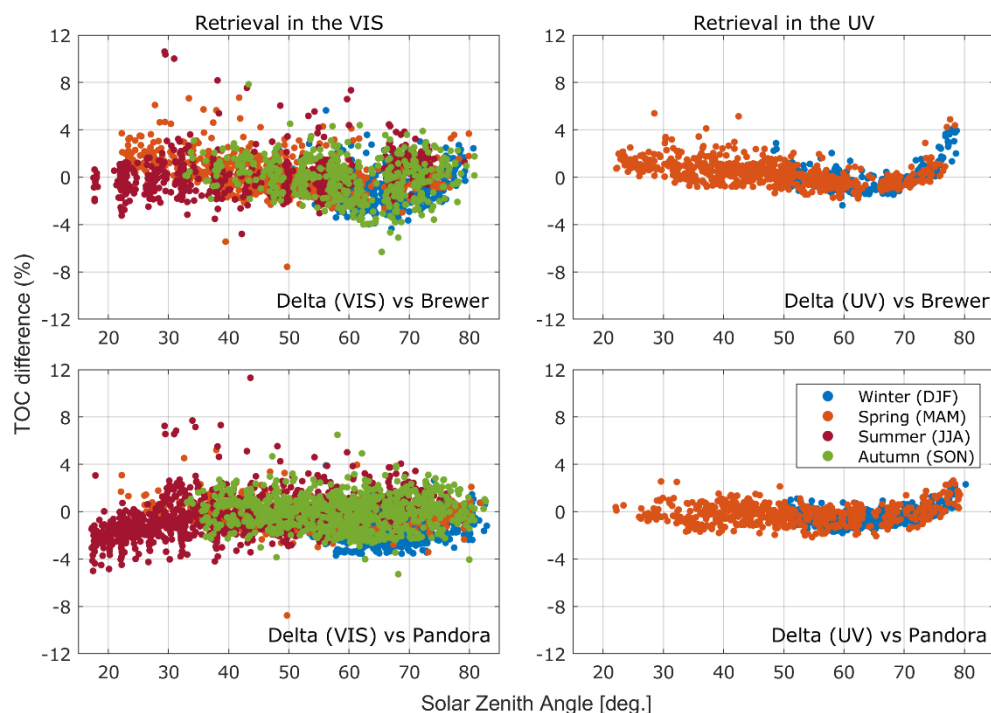
650 Figure 11: Seasonal dependence of TOC differences between Delta-Brewer, and Delta-Pandora as a function of SZA. The top row shows the percentage differences of Delta VIS (left) and Delta UV (right) with the Brewer, while the bottom row shows the corresponding differences with the Pandora. Note that no data are available in summer and autumn for the Delta UV dataset.
