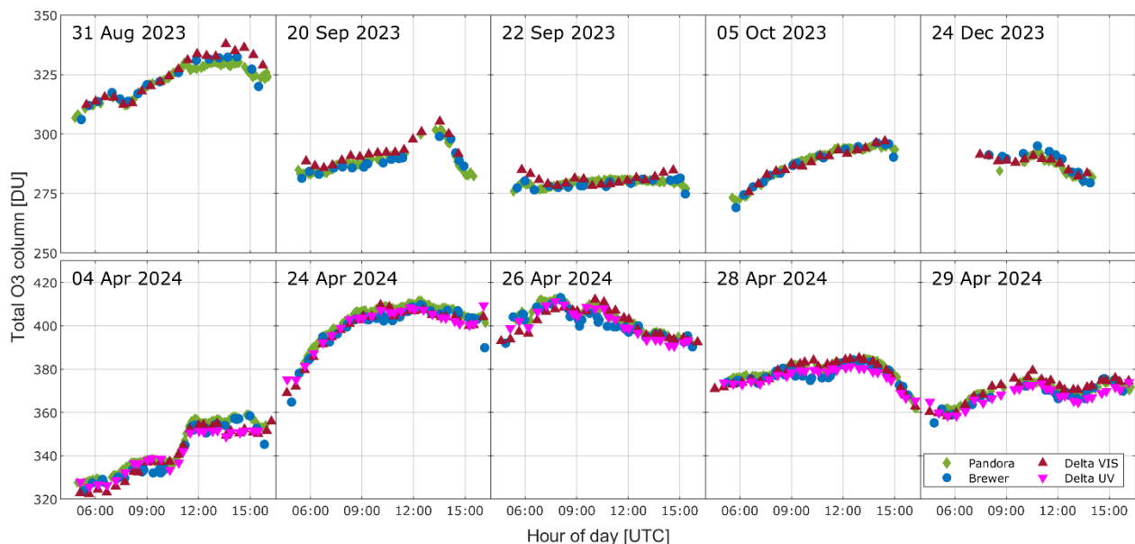
705 Figure 13: The diurnal variability of TOC captured by Pandora (green), Brewer (blue), Delta VIS (red) and Delta UV (magenta) for selected days.
