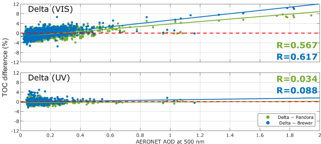
750 Figure 14: TOC differences of Delta from Pandora (green markers) and Brewer (blue markers) retrieved in the VIS (top panel) and the UV (bottom panel) spectral ranges as a function of AOD at 500 nm.
