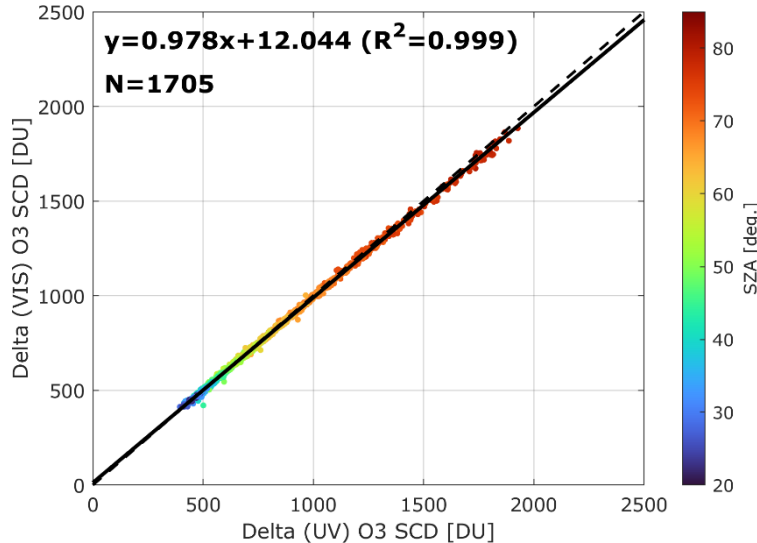
Figure 5: Comparison of ozone SCDs retrieved from Delta UV and VIS spectra over the study period. The data are color-coded by SZA. The dashed line represents the 1:1 reference, while the solid line shows the linear regression fit. N corresponds to the total number of Delta measurements.
