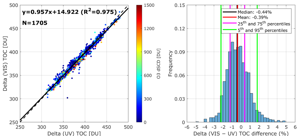
Figure 6: Comparison of TOC measurements from the UV and VIS channels of Delta over the study period. (left) Scatter plot of VIS against UV retrievals, color-coded by ozone dSCDs. The dashed line represents the 1:1 reference, while the solid line shows the linear regression fit. N corresponds to the total number of Delta measurements. (right) Frequency distribution of their respective percentage differences (VIS – UV). The vertical lines indicate the median (black), mean (red), the 25 th and 75 th percentiles (magenta), and the 5 th and 95 th percentiles (green).
