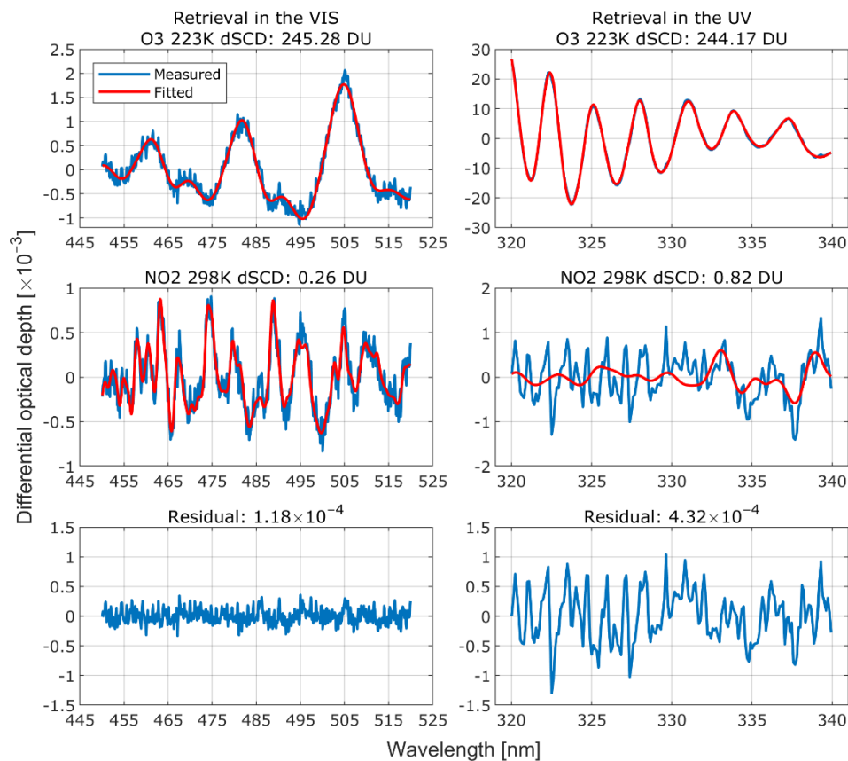
330 Figure 2: Example of DOAS spectral fitting for ozone in the VIS (left column) and UV (right column) spectral ranges. The top panels show the measured (blue) and fitted (red) differential optical depths for \text{O}_3 , the middle panels for \text{NO}_2 , and the bottom panels the corresponding fitting residuals.
