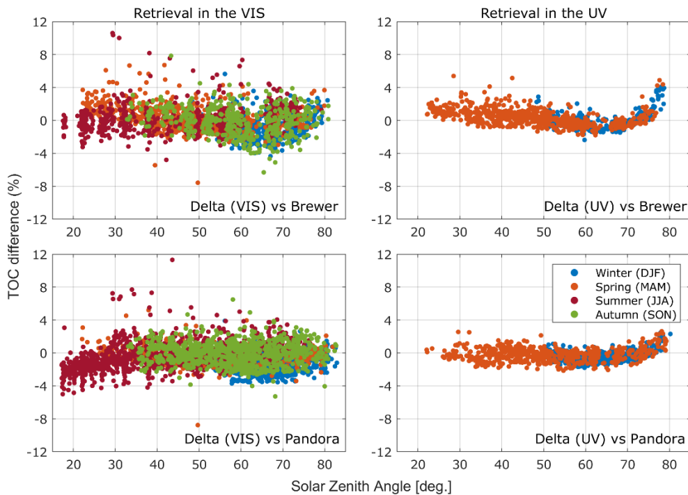
655 Figure 11: Seasonal dependence of TOC differences between Delta-Brewer, and Delta-Pandora as a function of SZA. The top row shows the percentage differences of Delta VIS (left) and Delta UV (right) with the Brewer, while the bottom row shows the corresponding differences with the Pandora (c and d). Note that no data are available in summer and autumn for the Delta UV dataset.
