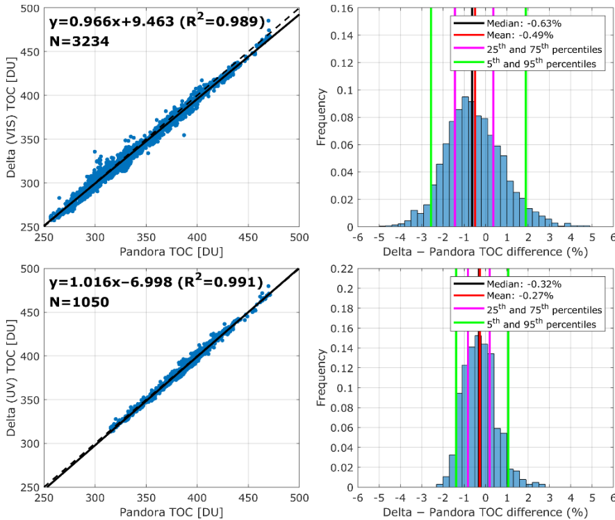
600 Figure 9: Same as Figure 8 but for the comparison of TOC measurements of Delta with Pandora.
