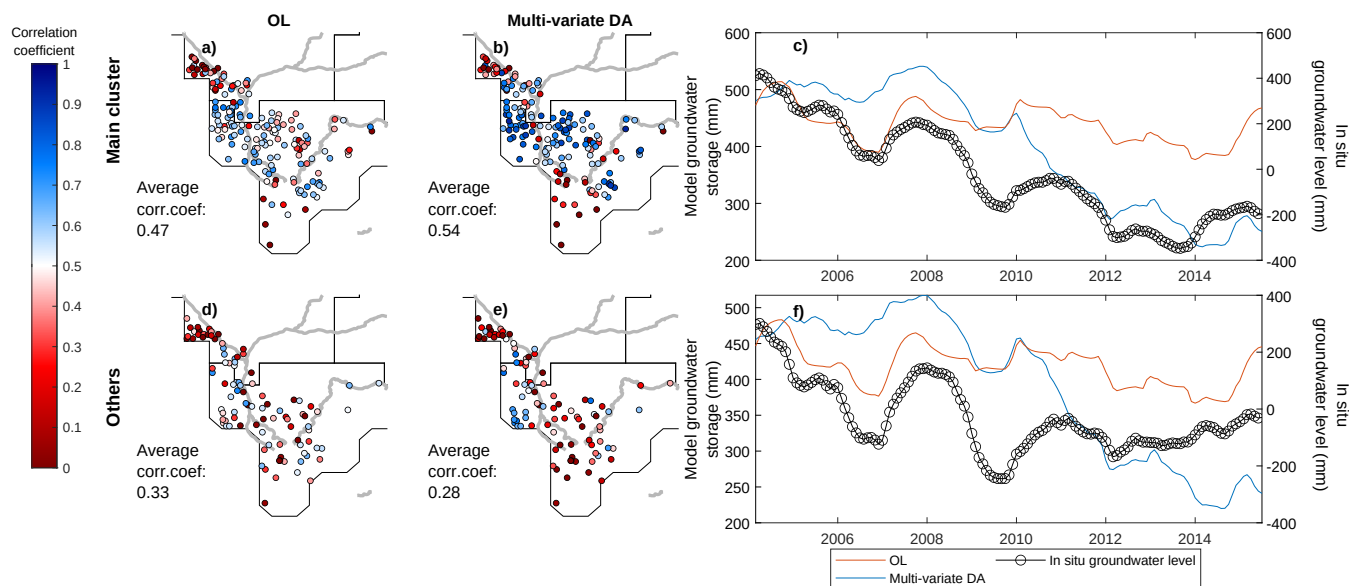
Figure 8. (a,b,d,e) Correlation coefficient between modeled groundwater storage and observed groundwater level for individual sites. The centerline of the main rivers of the region are added in the background as a reference. (c, f) Average groundwater storage and groundwater level time series for sites belonging to the main cluster (c) and remaining sites (f).
