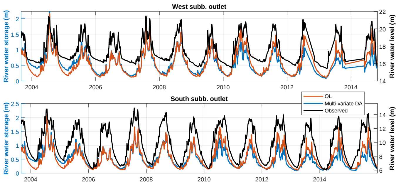
Figure 10. River water storage time series derived from OL (red) and multi-variate DA (blue), as well as in situ water level observations (black, with y axis on the right). The time series correspond to the two sites shown in Fig. 1.
