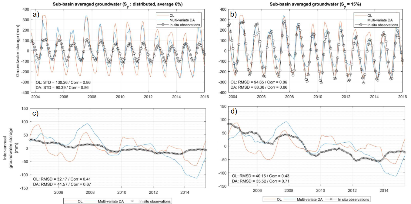
Figure 7. Inter-annual groundwater storage variability derived from OL, multi-variate DA and in situ groundwater level observations. a and b represent the time series, and c and d represent their inter-annual variability component. In a and c, the observed groundwater storage was computed using distributed yield values computed by Shamsudduha et al. (2011). In b and d, a uniform specific yield value of 15% was used.
