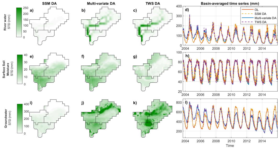
Figure 4. Standard deviation of DA minus OL on spatially distributed ( 0.1^\circ \times 0.1^\circ grid) model estimates for river water (a-c), SSM (e-g) and groundwater (i-k). The standard deviation is expressed in mm. The column in the right (d, h, l) shows basin-averaged time series for the same variables.
