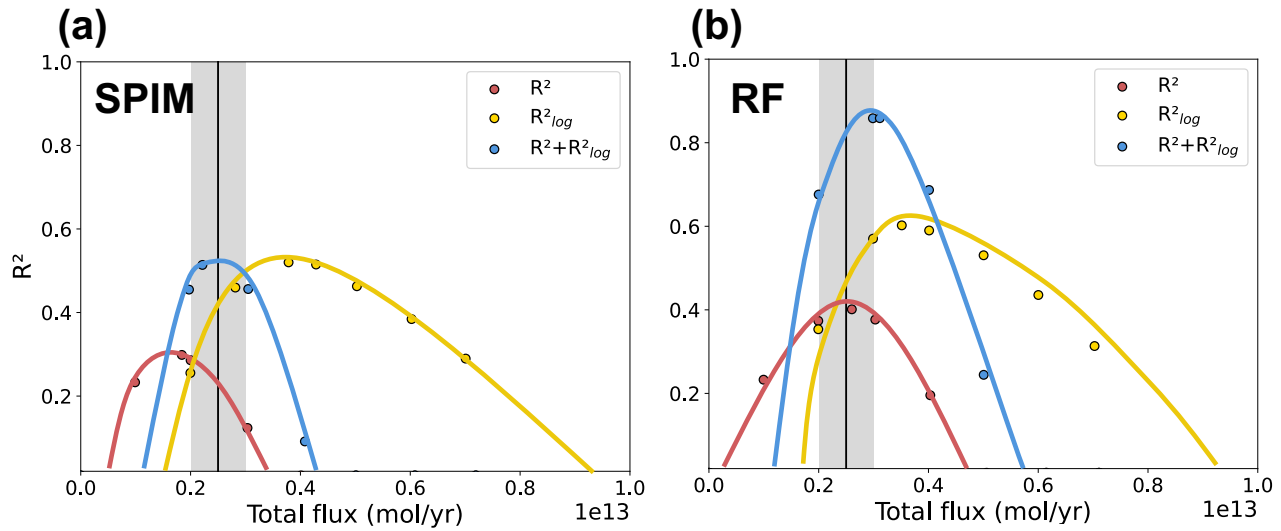
Figure 9: Result of parameter tests for GM09-SPIM and MErSiM.
