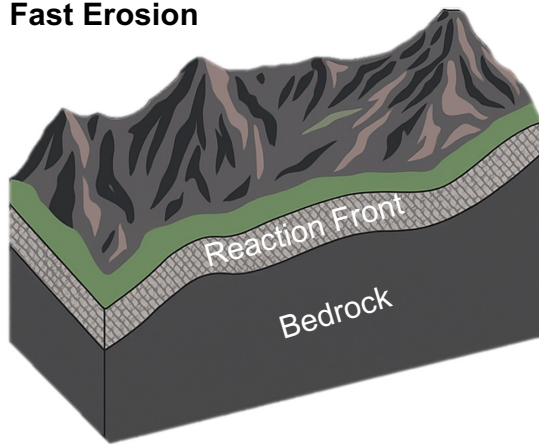
685 Figure 1: Conceptual diagram of the core of the GM09 model.
