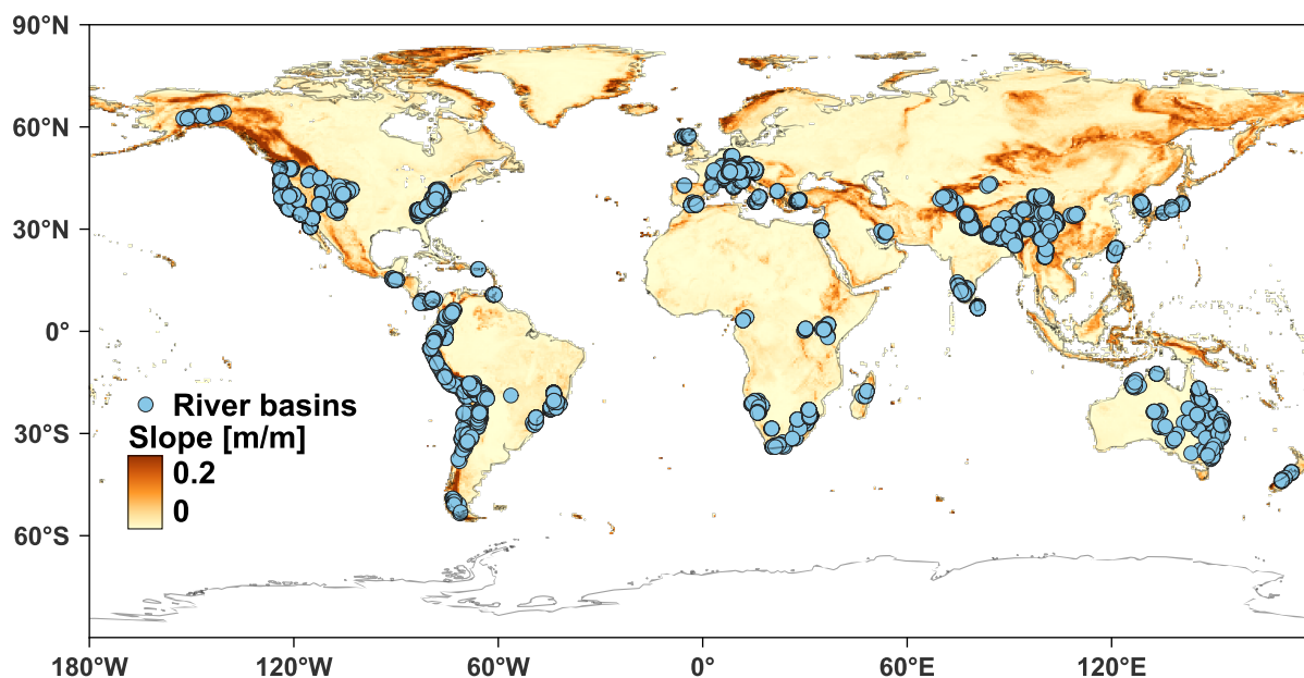
680 Figure 2: The geographical extent and distribution of global Be isotope erosion rate dataset.
