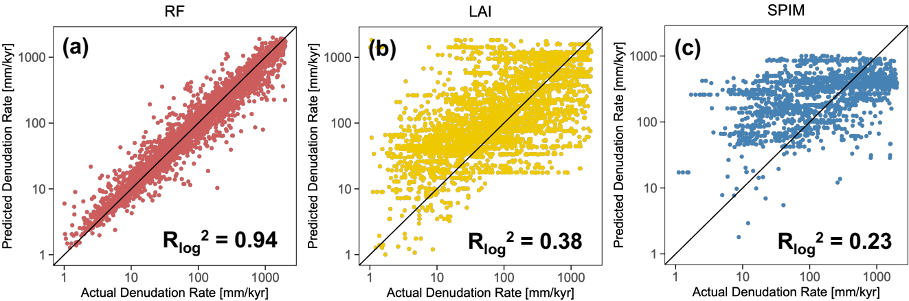
690 Figure 4: Scatter of predicted basin denudation rates by different methods vs. observations from OCTOPUS.
