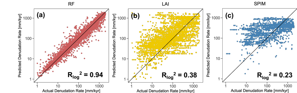
Figure 4: Scatter of predicted basin denudation rates by different methods vs. observations from OCTOPUS. The observed erosion rates are plotted against the model-predicted rates (y-axis) for (a) our Random Forest (RF) model, (b) the LAI-modified model from Zuo et al. (2024), (c) the original SPIM from Park et al. (2020). The diagonal line represents the 1:1 relationship. Both axes are on a logarithmic scale to accommodate the multi-order-of-magnitude range of erosion rates observed globally. The coefficient of determination for the logarithmic values ( R_{log}^2 ) is used as the primary metric of performance, indicating the proportion of variance in the observed data that is explained by the model. All the inputs of these models are from the same compilation of basin-average variable values.
