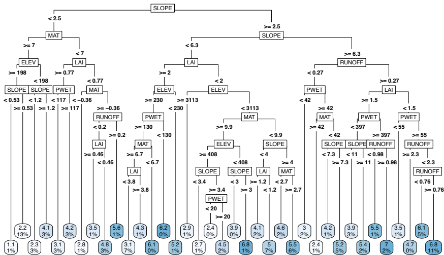
740 Figure 8: An example decision tree trained on training dataset (random 80% of the whole dataset).
