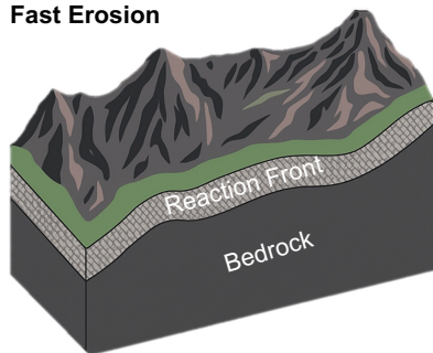
690 Figure 1: Conceptual diagram of the core of the GM09 model.
