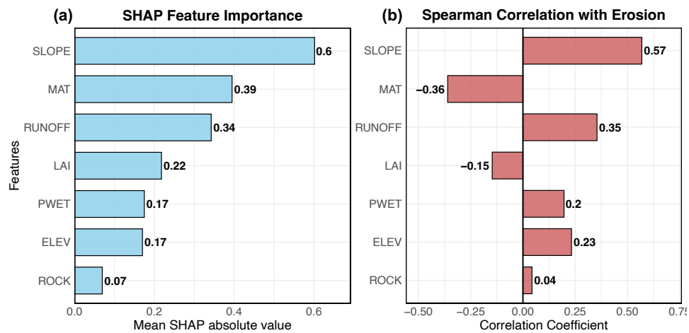
Figure 6: Importance and correlation of predictor variables.
