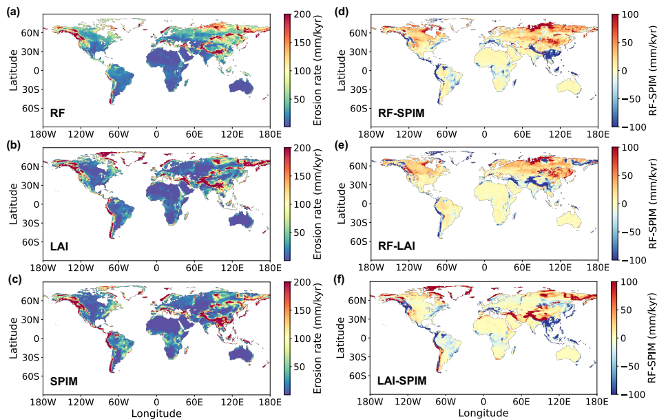
Figure 5: Global erosion rate map calculated by different erosion models and their differences.
