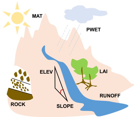
Figure 3: Cartoon showing the environmental factors that influence denudation rates.
