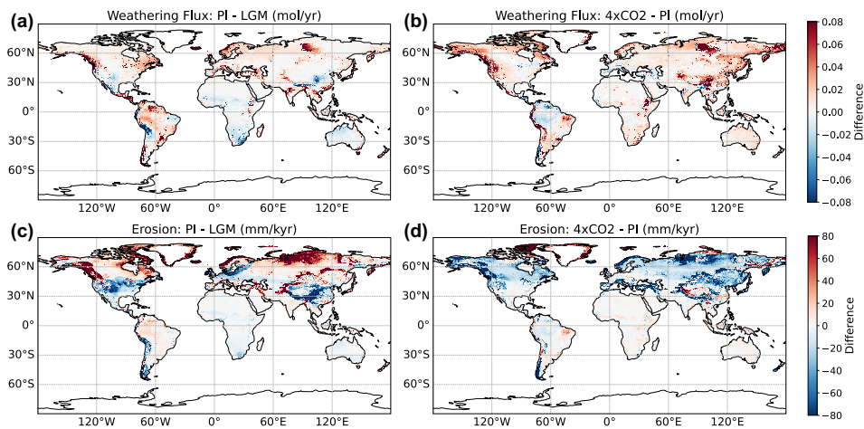
820 Figure 11: The difference of weathering and erosion for climate scenarios.
