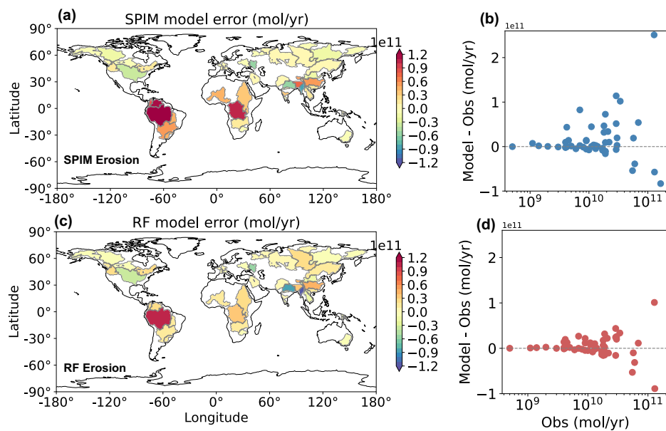
815 Figure 10: The difference (model – observation) in silicate weathering fluxes for 81 large rivers.
