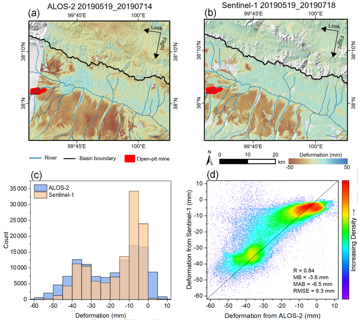
Figure 9. Comparison of surface deformation derived from ALOS-2 L-band and Sentinel-1 C-band data during a similar period of the thawing season in 2019: (a) ALOS-2-derived deformation from 19 May–14 July 2019; (b) Sentinel-1-derived deformation from 19 May–18 July 2019; (c) histogram distributions of the two deformation maps; (d) density scatter plot of the two deformation maps with the correlation and difference statistics, including correlation coefficient ( R ), mean bias (MB), mean absolute bias (MAB), and RMSE.
