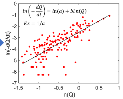
Figure 4. Schematic illustration of the link between permafrost hydrology and streamflow recession analysis. (a) Conceptual model of permafrost hydrology and changes in the streamflow recession process with permafrost degradation. (b) Recession period selection based on the daily discharge time series. (c) Linear fitting used to derive the recession parameters.
