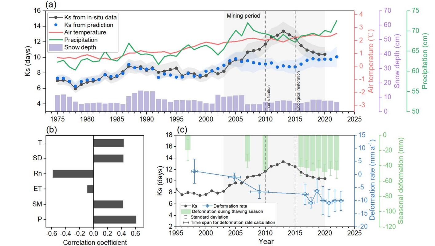
Figure 14. Long-term variations in the streamflow recession constant ( K_s ) with the variations in deformation rate and thaw-season deformation during different periods: (a) K_s derived from in-situ streamflow data and predicted from climatic variables along with key climatic variables: air temperature, precipitation and snow depth. The shaded bands indicate the 95% confidence intervals; (b) correlation between climatic factors and K_s before mining. Climatic factors including precipitation (P), soil moisture (SM), snow depth (SD), evapotranspiration (ET), net radiation (Rn) and air temperature (T); (c) regional mean deformation rate and thaw-season deformation within the overlapping deformation area observed by all sensors across the upper Datong River basin during different periods.
