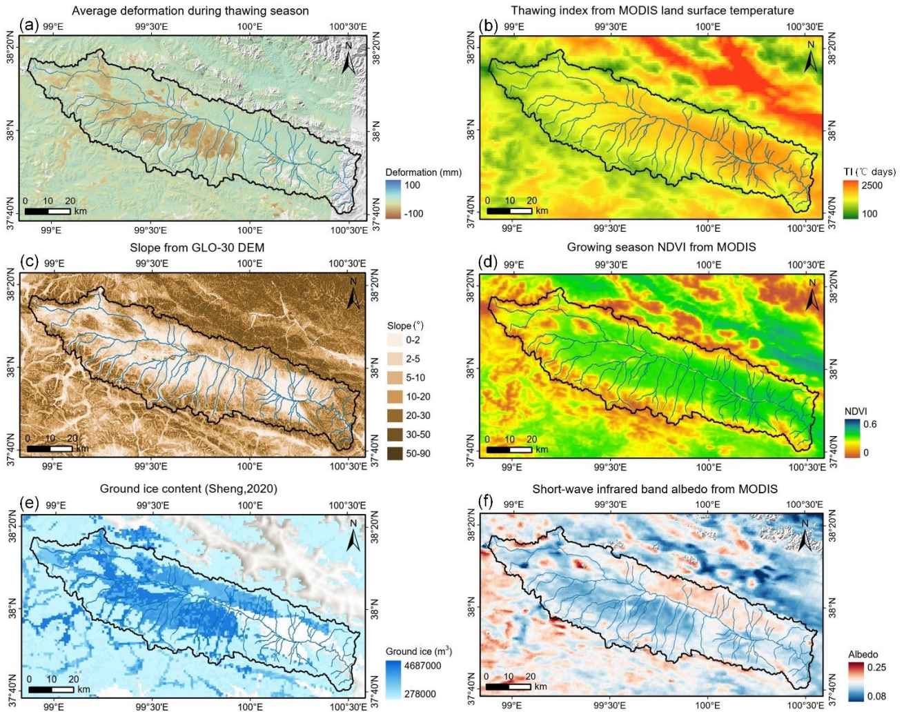
465 Figure 13. Comparison of the spatial distribution of environmental factors and thaw season deformation: (a) seasonal deformation maps derived using Sentinel-1 SAR data; (b) thawing index; (c) slope; (d) NDVI; (e) ground Ice Content; (f) shortwave infrared albedo.
