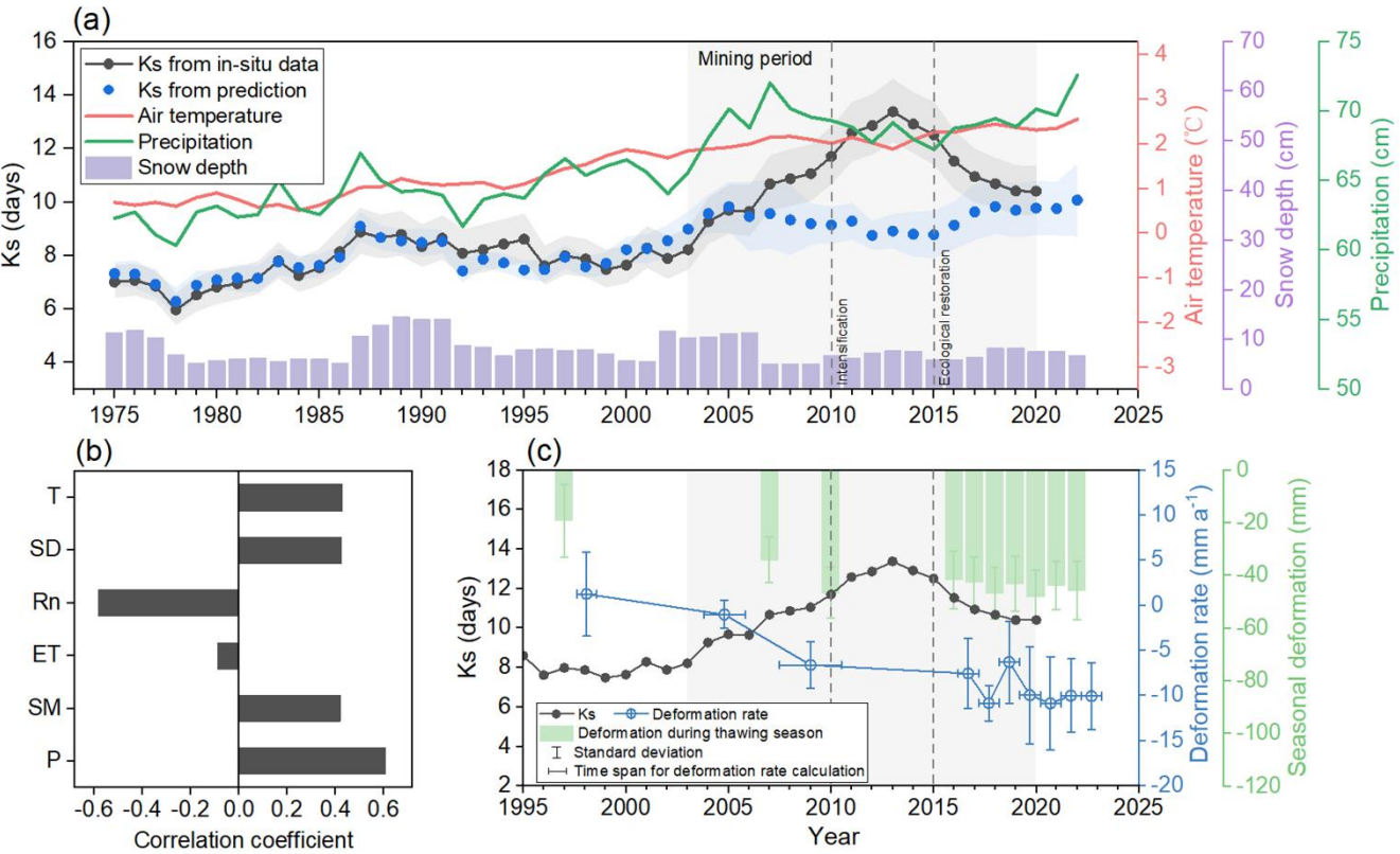
485 Figure 14. Long-term variations in the streamflow recession constant ( K_s ) with the variations in deformation rate and thaw-season deformation during different periods: (a) K_s derived from in-situ streamflow data and predicted from climatic variables along with key climatic variables: air temperature, precipitation and snow depth. The shaded bands indicate the 95% confidence intervals; (b) correlation between climatic factors and K_s before mining. Climatic factors including precipitation (P), soil moisture (SM), snow depth (SD), evapotranspiration (ET), net radiation (Rn) and air temperature (T); (c) regional mean deformation rate and thaw-season deformation within the overlapping deformation area observed by all sensors across the upper Datong River basin during different periods.
