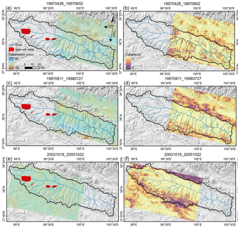
355 Figure 5. Surface deformation and coherence maps from early-stage C-band SAR acquisitions: ERS-2 (a–d) and Envisat (e–f). Positive deformation represents uplift, and negative deformation represents subsidence.
