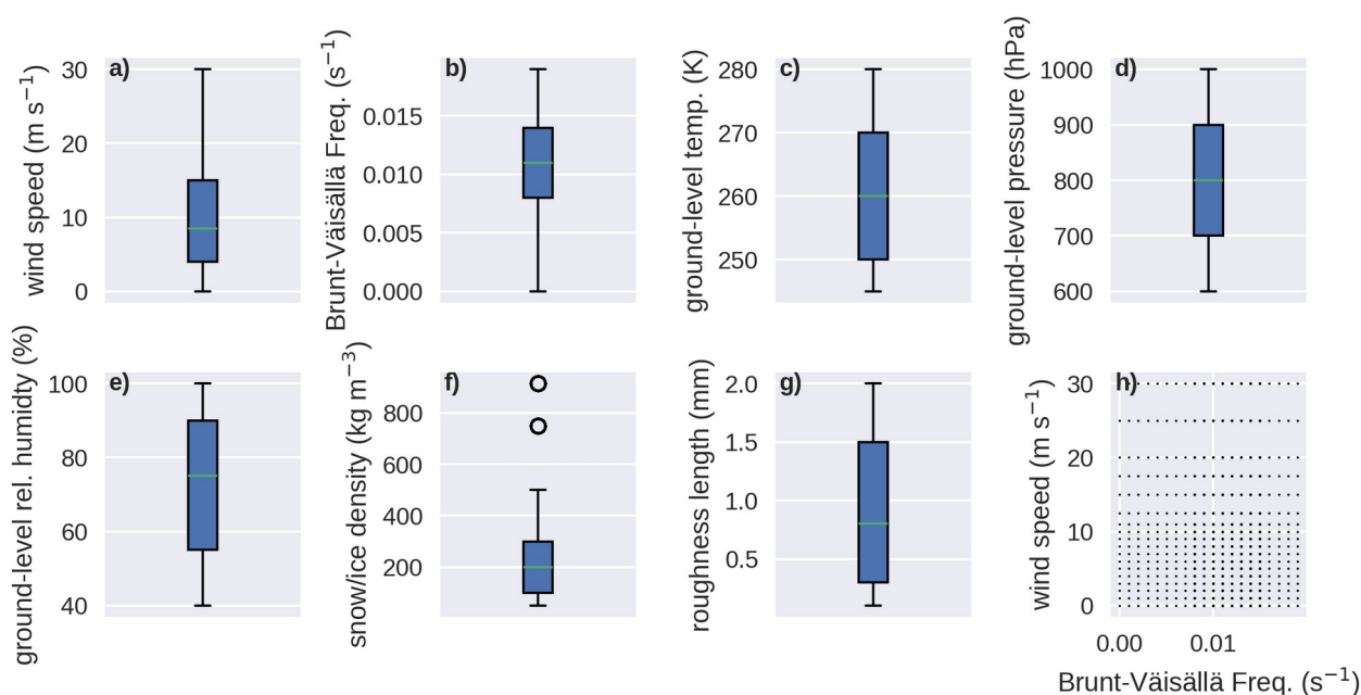
Figure R1: Reworked version of Figure 3 in the manuscript to also include combinations of wind speed and Brunt-Väisällä Frequencies used to drive the simulations of the training data set (h).
