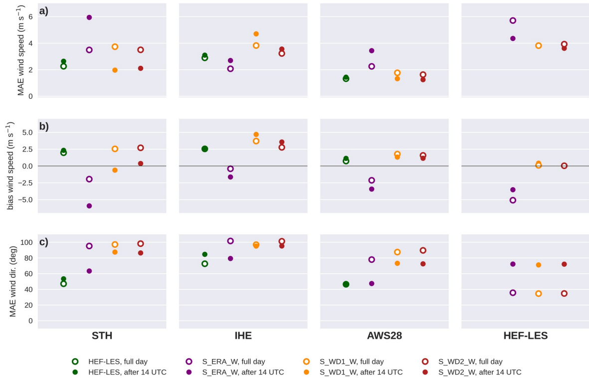
Figure R3: Similar to Fig. 11 of the manuscript, but with correction of the height difference between model output and observation, under the assumption of a neutral stratification.
