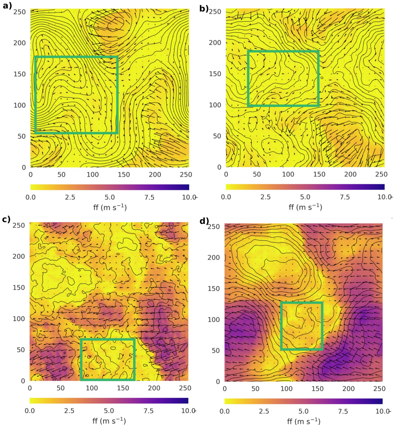
Figure R2: Examples for cases with chaotic, unsteady flow features: these regions are marked with a green rectangle.
