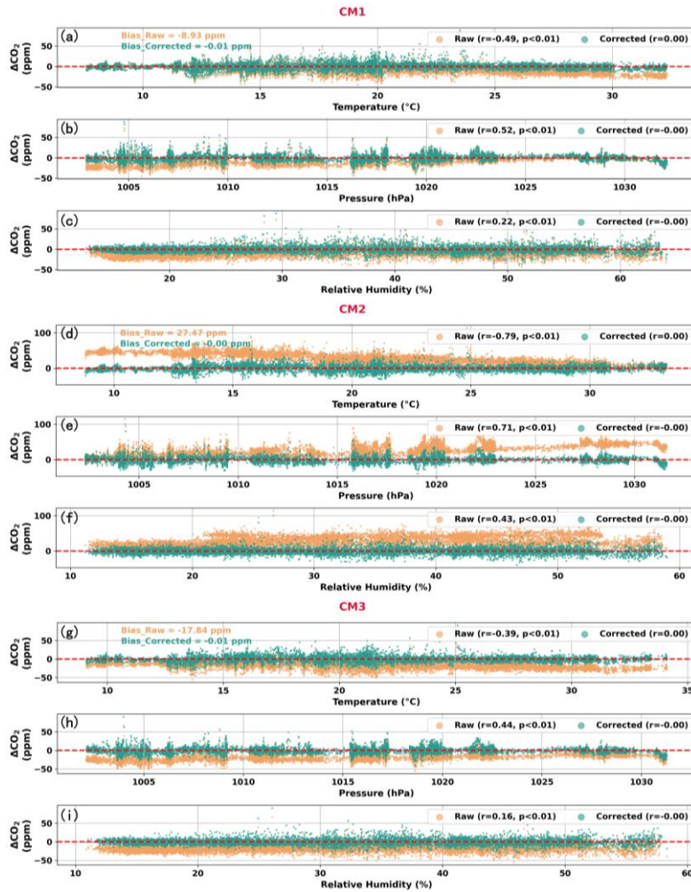
Figure 5: Variations of \Delta\text{CO}_2 ( \Delta\text{CO}_2=\text{CM-Picarro} ) for CM1 (a-c), CM2 (d-f), and CM3 (g-i) during land-based field observations, as functions of temperature (a, d, g), atmospheric pressure (b, e, h), and relative humidity (c, f, i). Orange dots represent data before environmental correction, while green dots represent data after environmental correction.
