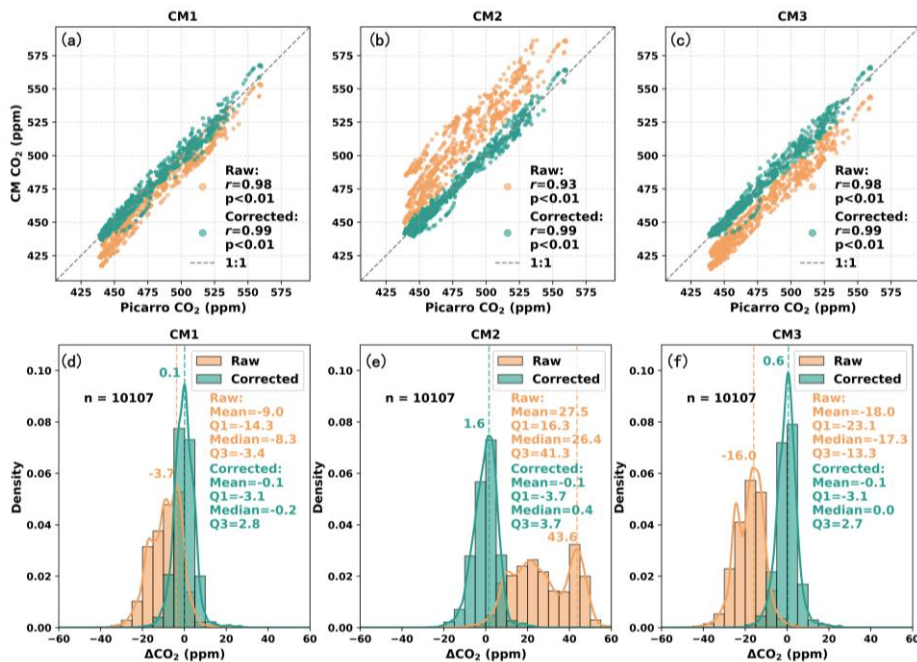
Figure 6: Direct comparison of hourly moving averages of CO 2 concentrations among CM1, CM2, CM3 and Picarro during land-based field observations (a-c), and histograms of ΔCO 2 distributions (d-f) (ΔCO 2 =CM-Picarro, where CM corresponds to CM1, CM2, and CM3, respectively). Orange dots and bars represent data before environmental correction, while green dots and bars represent data after environmental correction.
