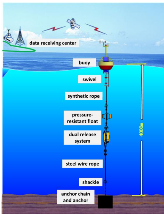
120 Figure 2: Schematic diagram of a deep-sea air-sea coupled monitoring buoy system
