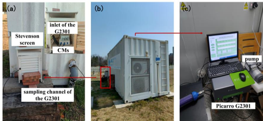
Figure 3: Land-based field observation experiments. (a) Configuration of CMs, Stevenson screen, and Picarro sampling channel. (b) Meteorological observation station, experimental cabin, and field deployment of CMs. (c) Field setup of the Picarro G2301.
