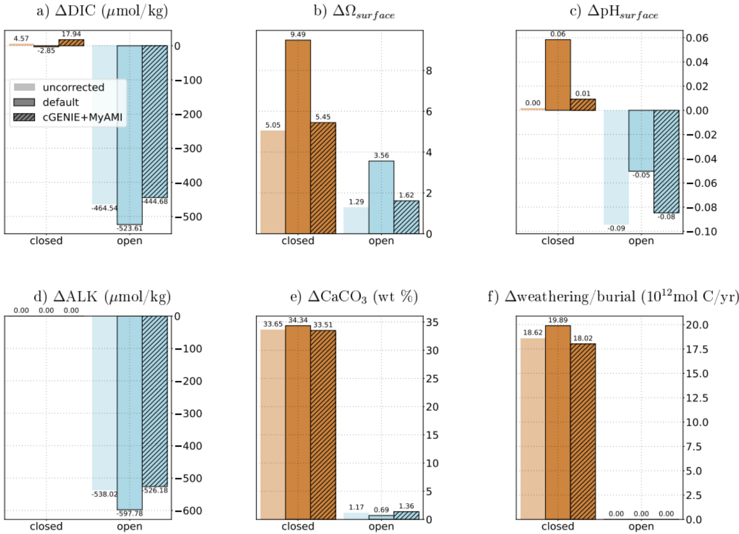
Figure 7: Effect of changing Mg/Ca from pre-industrial to Eocene-like for mean ocean DIC and ALK changes, mean surface pH and \Omega , average \text{CaCO}_3 content of marine sediments and total \text{CaCO}_3 burial in simulations without correcting for major ion changes, default cGENIE and cGENIE+MyAMI.
