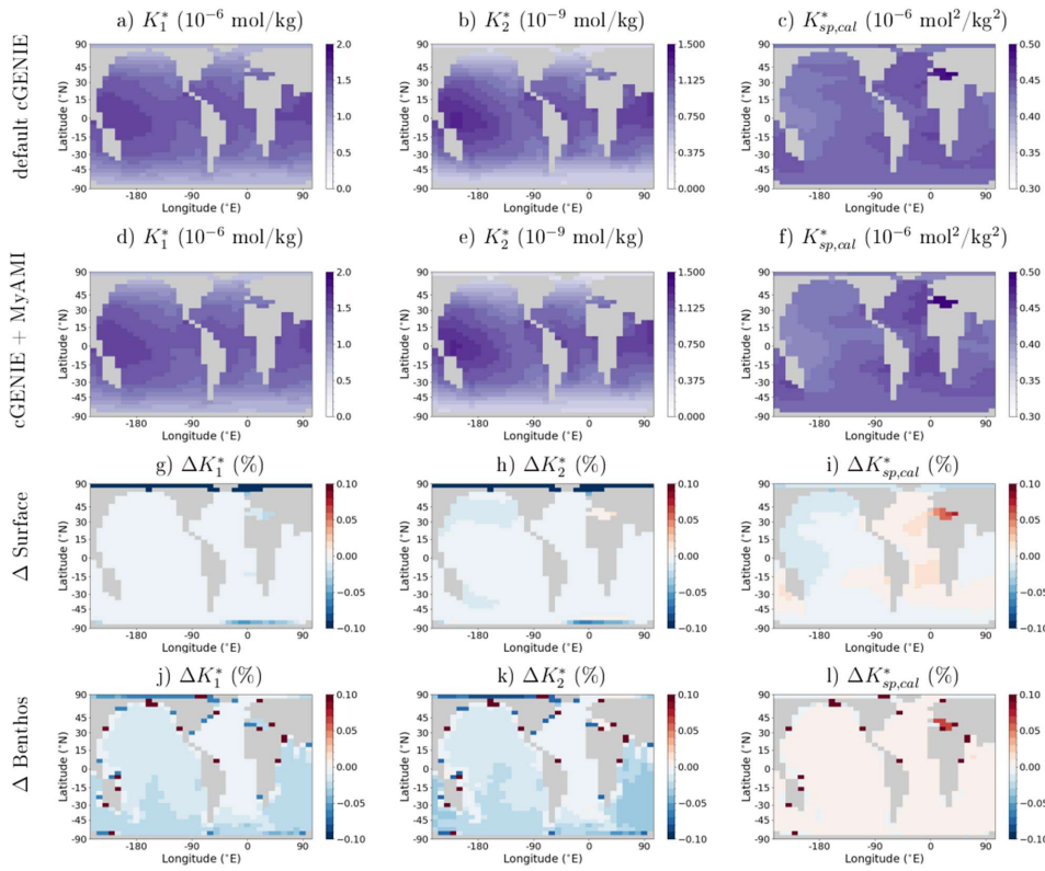
Figure 3: Absolute-surface ocean values of K_1^* , K_2^* , and K_{sp,cal}^* in default cGENIE (PI-BA-ocean) and cGENIE+MyAMI (PI-CB-ocean) solutions for the pre-industrial carbonate system (a-f) and difference between the two (simulations PI-CB-ocean minus PI-BA-ocean) for the surface and benthic ocean. The surface layer represents the uppermost 175 m of the water column and benthic values are from the deepest ocean grid box in every location. In the ‘ocean’ set up, organic and carbonate particles are instantaneously respired/dissolved when reaching the sediment-water interface. In shallow locations (less than 600 m water depth) where the particle flux is large, this results in unusual local carbonate system states that appear as brown cells in j-l.
