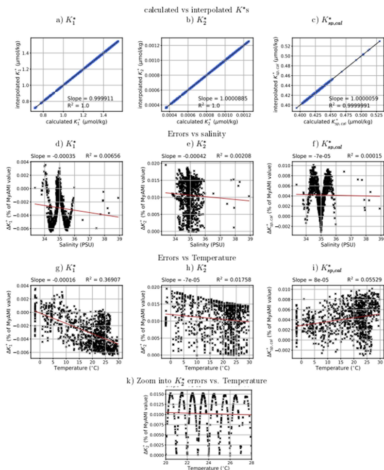
Figure 2: Errors due to interpolating rather than calculating in situ K^*_{s_i} in the surface ocean in simulation PIEE-CB-ocean . All errors are given as percentage of the exact MyAMI value.
