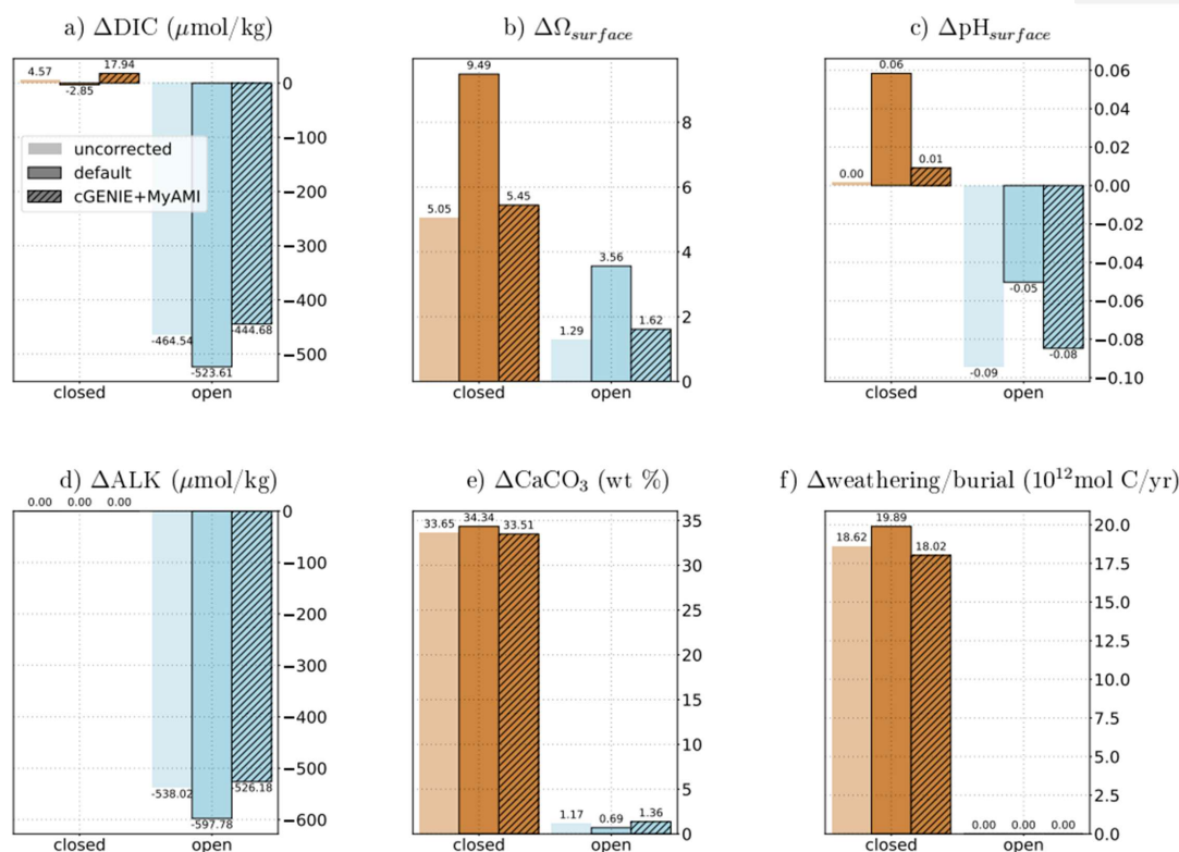
Figure 7: Effect of changing Mg/Ca from pre-industrial to Eocene-like for mean ocean DIC and ALK changes, mean surface \text{pH} and \Omega , average \text{CaCO}_3 content of marine sediments and total \text{CaCO}_3 burial in simulations without correcting for major ion changes, default cGENIE and cGENIE+MyAMI.
