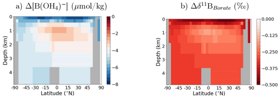
Figure 8: Zonally-averaged profiles of differences in borate ion concentrations and \delta^{11}\text{B} of borate derived from K^*_\text{B} and \text{pH} between cGENIE+MyAMI and default cGENIE (simulations EE-CB-open minus EE-BA-open) for the Pacific. The underlying pH differences are shown in Fig. SI.5c.
