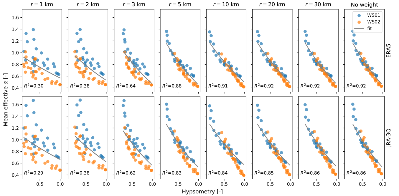
Figure A2. Mean observed effective values and calibration fit of the factor \alpha_{\text{exp}}(h) for different radii and both reanalysis products.
