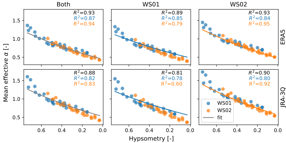
Figure B1. Mean observed-effective and modelled values of the factor \alpha(h) for a calibration over both valleys, or each valley individually, and for both reanalysis products.
