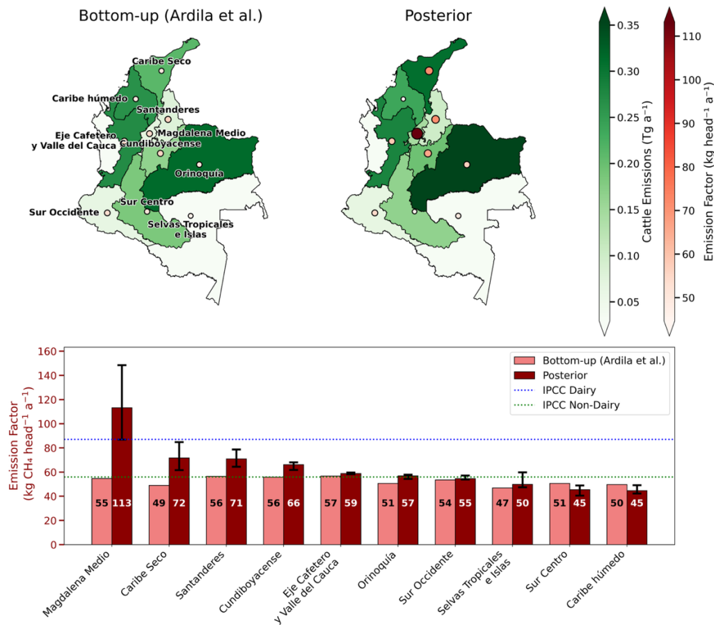
455 Figure 9: Cattle emissions and emission factors (EFs) for Colombia's ten IPCC Tier 2 regions. The top panels show the total emissions in each region and the inferred emission factors (emissions divided by the number of cattle) for both the bottom-up estimate from Ardila et al. (2025a) and the posterior estimate. The marker size corresponds to the emission factor. The bottom panel shows the same bottom-up and posterior EFs for each region as red bars. The error bars denote the range of posterior estimates from the inversion ensemble. Dotted lines show average IPCC Tier 1 enteric fermentation emission factors for Latin America for dairy and non-dairy cattle.
