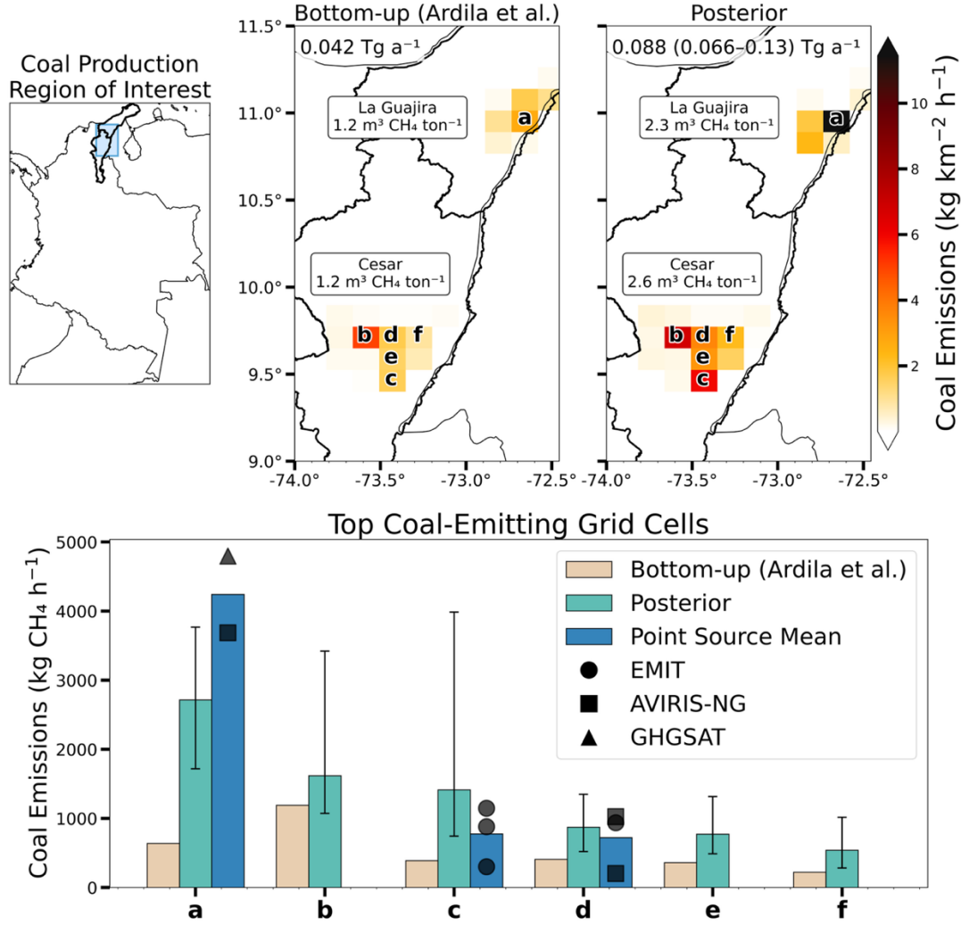
Figure 11: Coal mine emissions in the Cesar and La Guajira provinces. Posterior emissions on the 0.125^\circ \times 0.15625^\circ inversion grid are compared to the Ardila et al. (2025a) bottom-up inventory, which updates the BUR to account for declining coal production, and to point source observations. All emissions are from open-pit mines. The letters (a-f) shown on the maps correspond to the locations of the emissions shown on the bottom panel bar chart. Error bars on the posterior estimates show the ranges across the inversion ensemble. The blue bars indicate the means of multiple point source observations in a grid cell.
