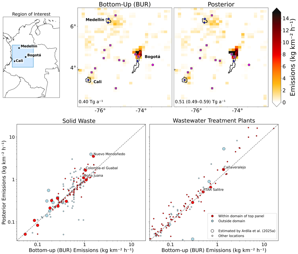
Figure 9: Emissions from solid waste and wastewater treatment plants in Colombia on the 0.125^\circ \times 0.15625^\circ grid of the inversion. The top panels show bottom-up (BUR) and posterior emissions for the west-central region including Bogotá, Medellín, and Cali, which accounts for 65% of national posterior emissions. Pink and blue crosses and pluses mark major landfills and wastewater treatment plants, respectively, identified by Ardila et al. (2025a); a pink dot indicates a landfill plume observed by EMIT. Region totals inset represent all waste emissions in the plotted domain ( 2.1^\circ to 6.9^\circ latitude, -77.1^\circ to -72.5^\circ longitude), with parentheses indicating the range across the inversion ensemble. The bottom panels are scatterplots of posterior versus bottom-up solid waste and wastewater emission estimates for individual grid cells, generally representing individual facilities. Facilities with emissions estimated by Ardila et al. (2025a) have larger symbols; additional sites from the Superintendent of Public Services and EDGARv8 are shown in red (if within the Bogotá–Medellín–Cali domain) or light blue (if outside). Major Ardila et al. (2025a) facilities within the Bogotá–Medellín–Cali domain with emissions above 0.5 \text{ kg km}^{-2} \text{ h}^{-1} are labeled.
