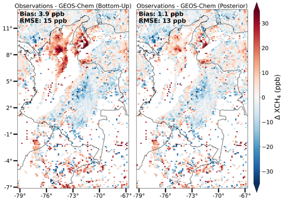
Figure 6: Optimization of 2023 methane emissions over Colombia on the 0.125^\circ \times 0.15625^\circ grid. Prior bottom-up emissions for Colombia are as given in Table 1 and shown in Figure 2 for anthropogenic sectors and Figure 4 for wetlands (GLWD+LPJ). Anthropogenic emissions outside Colombia are from GFEIv3 for fuel, EDGARv7 for livestock, ResME for hydroelectric reservoirs, and EDGARv8 for all other sectors. Posterior emissions are from our base inversion of TROPOMI+GOSAT observations. Total Colombia emissions and their anthropogenic component are inset. The right panel gives the ratio of posterior to prior bottom-up emissions. Grid cells with near-zero bottom-up emissions are shown in white in all panels.
