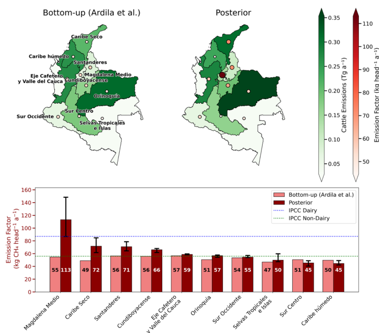
480 Figure 9: Cattle emissions and emission factors (EFs) for Colombia's ten IPCC Tier 2 regions. The top panels show the total emissions in each region and the inferred emission factors (emissions divided by the number of cattle) for both the bottom-up estimate from Ardila et al. (2025a) and the posterior estimate. The marker size corresponds to the emission factor. The bottom panel shows the same bottom-up and posterior EFs for each region as red bars. The error bars denote the range of posterior estimates from the inversion ensemble. Dotted lines show average IPCC Tier 1 enteric fermentation emission factors for Latin America for dairy and non-dairy cattle.
