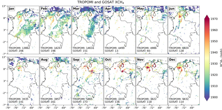
Figure 5: Atmospheric methane concentrations from TROPOMI and GOSAT over the inversion domain in 2023. Mean dry-column methane mixing ratios ( \text{XCH}_4 ) are shown on the native inversion grid ( 0.125^\circ \times 0.15625^\circ ) for each month, with the number of observations given in each panel.
