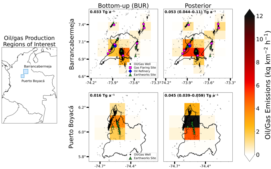
Figure 11: Bottom-up (BUR) and posterior oil/gas emissions in the oil production regions of Barrancabermeja and Puerto Boyacá that account for 82% of the national upward adjustment to oil/gas emissions in the inversion. Totals shown are for all oil/gas emissions in each domain (6.6° to 7.6° latitude, -74.25° to -73.25° longitude for Barrancabermeja, 5.7° to 6.4° latitude, -74.8° to -74.1° longitude for Puerto Boyacá). Black dots, pink squares, and blue diamonds indicate the locations of wells, gas flaring sites, and oil refineries, respectively, identified from the OGIM database (Omara et al., 2023). Green triangles indicate the locations of leaking, venting, or flaring infrastructure documented by Earthworks using shortwave infrared (SWIR) cameras (Anon, 2023).
