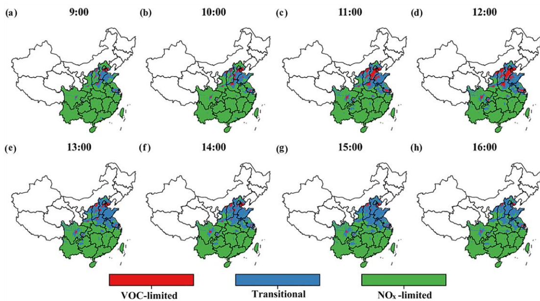
Figure 7. Diurnal photochemical-regime classification over study areas in O 3 pollution period from April to September 2023. (a-h) the analysis utilizes eight-hourly HCHO/NO 2 ratio data from the GEMS satellite to classify the regional O 3 formation dynamics in polluted areas (regions with GEMS NO 2 columns exceeding 1.0 \times 10^{15} molec·cm -2 ). The classification thresholds for VOC-limited, transitional, and NO x -limited conditions are based on the relationship between hourly surface high O 3 occurrence probabilities and GEMS HCHO/NO 2 , as shown in Figure 4 .
