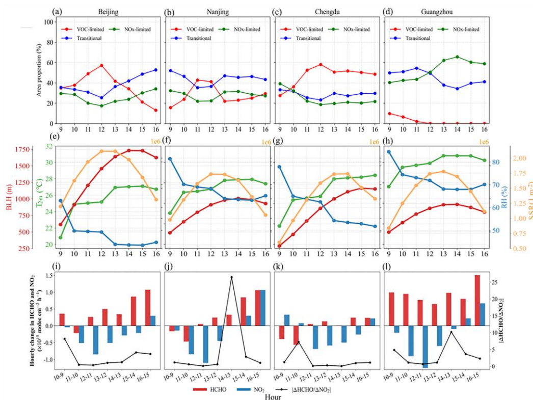
Figure 9. Hourly-averaged diurnal variations of ozone formation regimes, meteorological conditions, and precursor concentration for representative cities during the warm season from 2021 to 2023: Beijing (a, e, i), Nanjing (b, f, j), Chengdu (c, g, k), and Guangzhou (d, h, l). (a–d) fractional contributions of \text{O}_3 formation regimes. (e–h) hourly time series of meteorological variables (BLH, T_{2m} , RH, SSR). (i–l) hourly rates of change in \Delta\text{HCHO} and \Delta\text{NO}_2 .
