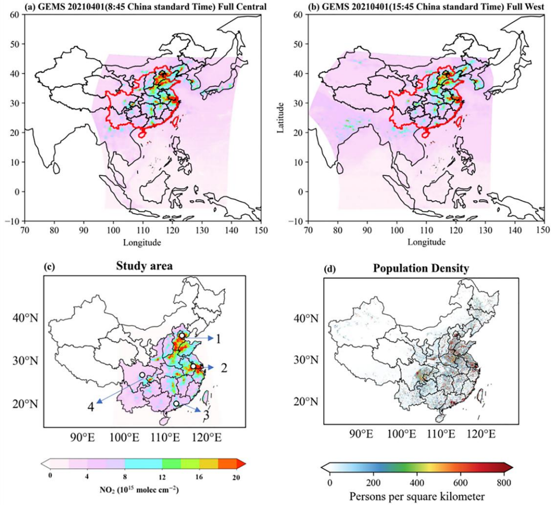
Figure 1. (a) NO 2 in the Full Central (FC) region as inverted by GEMS satellite at 8:45 LST on April 1, 2021. (b) NO 2 in the Full West (FW) region as inverted by GEMS satellite at 15:45 LST on April 1, 2021, and (c) the study area of this study (the red combined region in panel (a)), where regions 1–4 denote the BTH, YRD, PRD, and SC regions, respectively. The white circular symbols from north to south indicate Beijing, Nanjing, Chengdu, and Guangzhou. (d) Spatial distribution of population density in China, 2017, the population data for the study area (a red ensemble area) represents approximately 87% of the country's total population.
