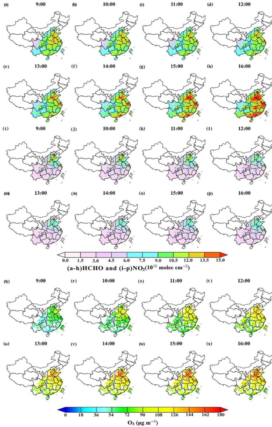
Figure 2. Hourly atmospheric monitoring in China during the warm season (April to September 2021-2023). (a-h) and (i-p) Spatial distribution of hourly mean HCHO and NO 2 levels retrieved from GEMS satellite data. (q-x) Temporal variations in ground-level mean O 3 concentrations, observed at various monitoring stations.
