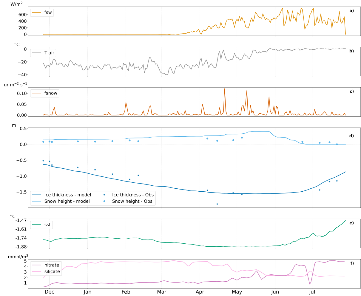
Figure 3. Overview of the forcing for the MOSAiC study case. Atmospheric forcing: a) downward shortwave radiation (fsw), b) 2 m atmospheric temperature ( T_{\text{air}} ), and c) precipitation (fsnow). Panel d) shows snow height and ice thickness as simulated by CICE + Icepack (line) together with observations collected during the coring events at the FYI site (dots/stars). Oceanic forcing: e) sea surface temperature (sst), and f) nutrients concentration in the water.
