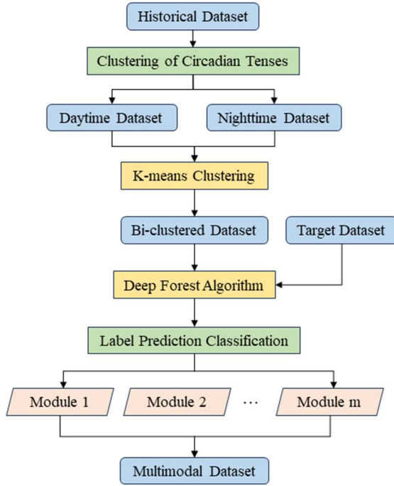
Figure 4: BCMC model flow diagram.
