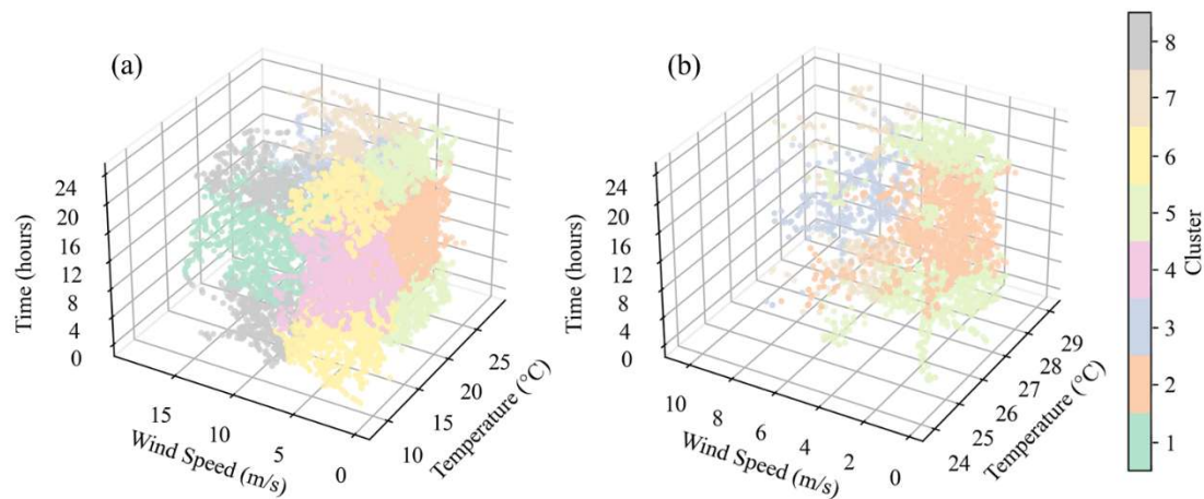
Figure 6: Results of the BCMMC model. (a) Bi-clustering classification, and (b) label
