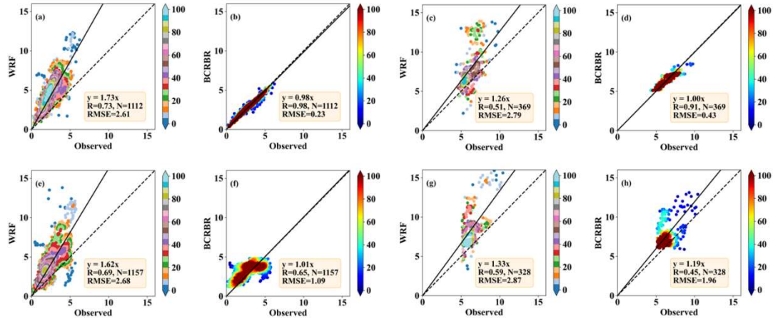
Figure 10: Regression scatter density plots for WRF forecast and the forecast of the BCRBR model. (a), (c), (e), (g) represent patterns 1, 2, 3, 4 respectively for WRF, and (b), (d), (f), (h) represent patterns 1, 2, 3, 4 respectively for BCRBR.
