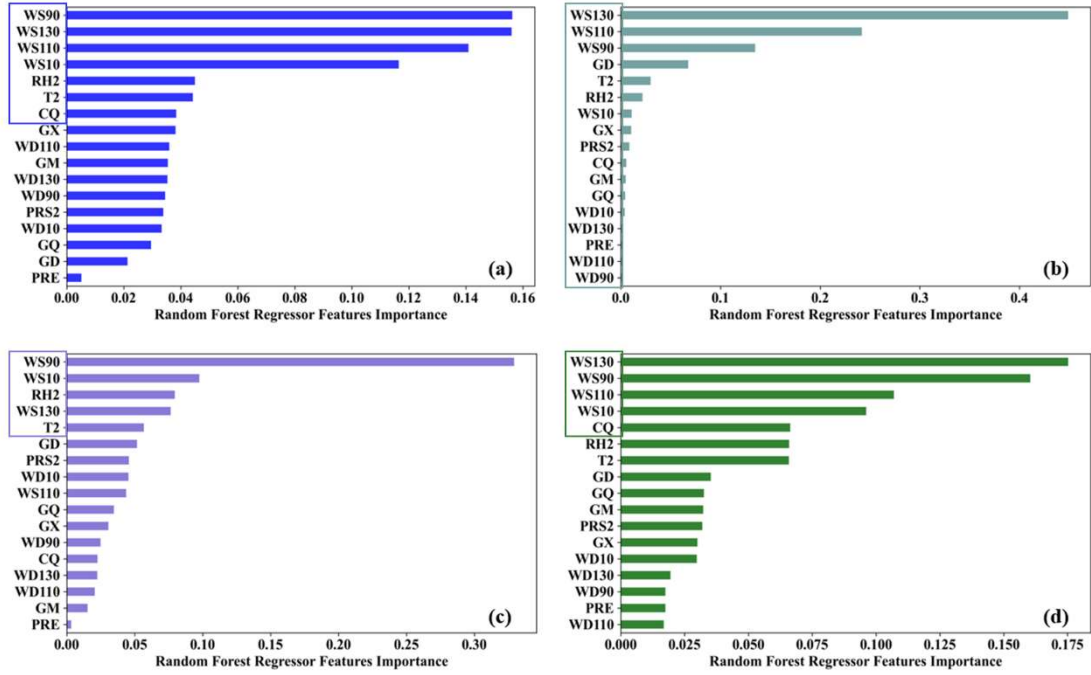
Figure 8: Importance of the 4 patterns. (a), (b), (c), and (d) represent patterns 1, 2, 3, and 4 respectively. The framed features represent the final input.
