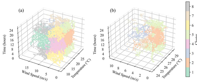
Figure 6: Results of the BCMC model. (a) Bi-clustering classification, and (b) label prediction.
