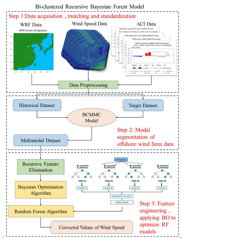
Figure 1: BCRBR model flow diagram to correct for predicted wind speed by WRF.
