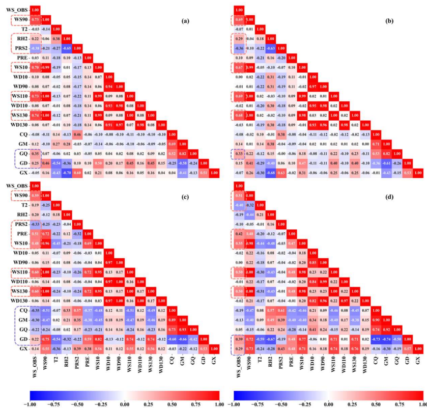
Figure 7: Correlation between variables of the 4 patterns. (a), (b), (c), and (d) represent patterns 1, 2, 3, and 4 respectively. The red dashed boxes represent highly relevant meteorological elements; blue dashed boxes represent highly relevant ACI.
