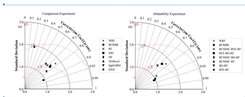
Figure 13: Taylor diagrams of the predictions of August 2023 for each model. (a) Comparison experiment, (b) ablative experiment.
