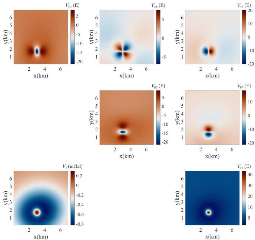
418 Figure 12: The gravity field and gradient components generated by the salt dome model using G&M3D 1.0. Here, 1 mGal = 10^{-5} m·s -2 and 1 E = 10^{-9} s -2 .
