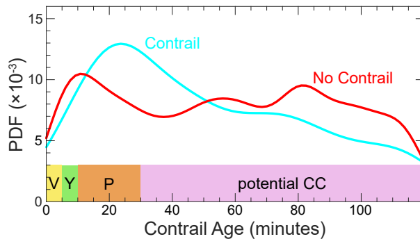
Figure 11. Probability density functions (PDF MS:s ) of the time delay between the passage of an aircraft through a cirrus cloud and the WALES lidar observation as a measure of contrail age. Data refer to the circles in MS: Figures Figs. 9 and 10 but for all WALES observations during ML-CIRRUS and CIRRUS-HL (see also Table 2). The colored bars mark different stages of the contrail life cycle: vortex phase (V, yellow), young contrails (Y, green), persistent contrails (P, orange), and rev2: potential contrail cirrus ( rev2: potential CC, magenta) rev2: that can form when persistent contrails are spread out spatially as a result of wind shear.
