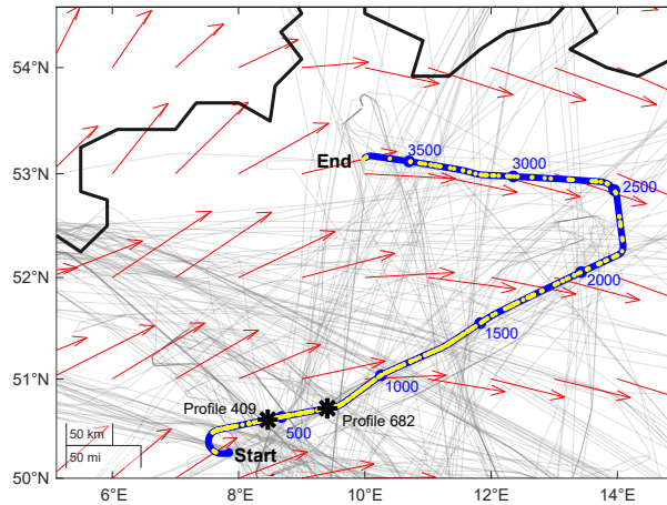
Figure 5. Overview of the location of about 1 h of WALES measurements along the HALO route (blue line with blue dots indicating intervals of 500 profiles) around noon on 1 April 2014 (magenta in Figure Fig. 1). The yellow dots mark the location of advected intercept points with commercial aircraft passing through the region (thin gray lines) less than 2 h prior to the HALO observation (see Section Sect. 2.4). The ERA5 wind field is indicated by red arrows. Black rosettes highlight the location of the profiles shown in Fig. 7.
