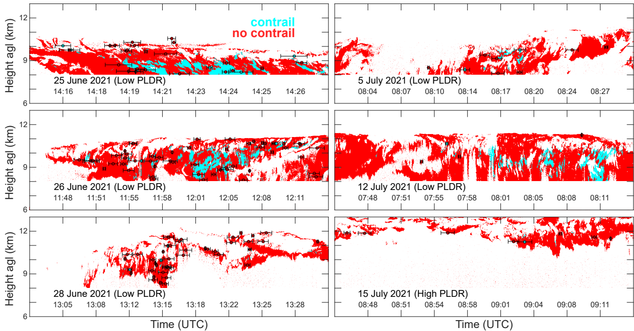
Figure 10. Same as rev3:FigureFig. 9 but for WALES observation of cirrus clouds during CIRRUS-HL and with orange regions in Fig. 9 reassigned to unperturbed cloud (red). Note that gaps in the cloud area at 10 to 12 km between 13:15 and 13:29 MS UTC on 28 June 2021 are due to detector saturation for signals from optically thick regions of the cloud.
