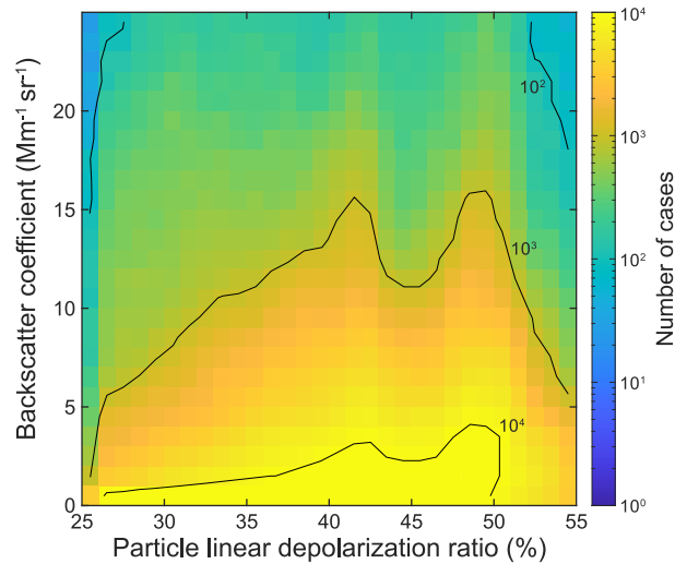
Figure 2. 2d histogram MS:s of rev2: particle backscatter coefficient ( \beta ) and rev2: particle linear depolarization ratio ( \delta ) for the WALES cirrus observations during ML-CIRRUS.
