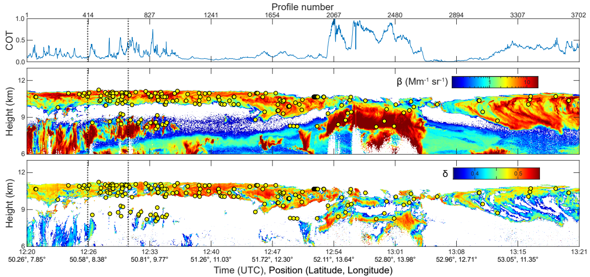
Figure 6. Lidar observation during 1 April 2014 with intersection-advected intercept points (yellow dots): (a) cloud optical thickness, (b) backscatter coefficient, (c) particle linear depolarization ratio. The dotted lines mark the location of the profiles shown in Figure 7 .
