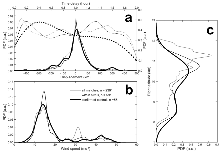
Figure A1. Probability density functions (PDF MS:s , in arbitrary units) of the occurrence of different aircraft-HALO intercept cases (all: thin MS: greygray lines, within cirrus: thin black lines, and confirmed contrail: bold black lines) during ML-CIRRUS (see Table 2) with respect to (a) time delay (dotted) and corresponding displacement (solid), (b) wind speed at flight altitude, and (c) flight altitude.
