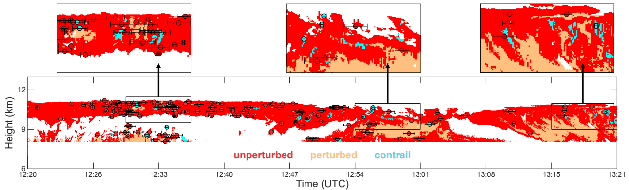
Figure 9. MS: Result of applying the contrail mask to the observations in Figure 6. Unperturbed cirrus regions identified in step one are marked in red. Perturbed cloud regions that pass the \beta - \delta threshold (step one) but fail the heterogeneity criterion (step two) are marked orange here but re-labelled as unperturbed cirrus in the final masking. Perturbed cloud regions passing the heterogeneity test are marked in cyan. Dots refer to the matched cases in Figure 6 that have been confirmed as contrails (cyan) or unperturbed cloud (red) in the manual analysis. The insets in the top row represent close-ups of the regions marked by black boxes in the bottom panel. rev3: Result of applying the contrail mask to the observations in Fig. 6. Unperturbed cirrus regions identified in step one are marked in red. Perturbed cloud regions that pass the \beta - \delta threshold (step one) but fail the heterogeneity criterion (step two) are marked orange here but re-labeled as unperturbed cirrus in the final masking. Perturbed cloud regions passing the heterogeneity test are marked in cyan. Dots refer to the matched cases in Fig. 6 that have been confirmed as contrails (cyan) or unperturbed cloud (red) in the manual analysis. Error bars represent the range of intercept locations related to assuming an error of 1 \text{ m s}^{-1} in ERA5 wind speed. The insets in the top row represent close-ups of the regions marked by black boxes in the bottom panel.
