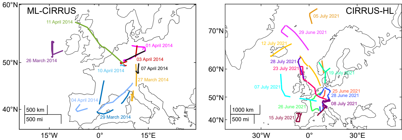
Figure 1. Segments of HALO flight paths with WALES lidar measurements during ML-CIRRUS in March and April 2014 (left) and during CIRRUS-HL in June and July 2021 (right) with MS: colours MS: colors referring to different days.
