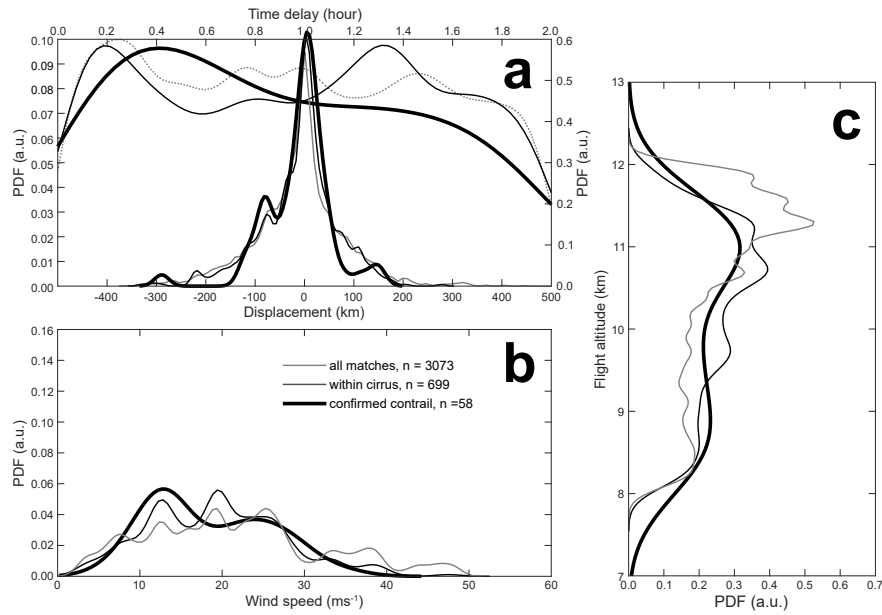
Figure B1. Probability density functions (PDF MS:s , in arbitrary units) of the occurrence of different aircraft-HALO intercept cases (all: thin grey lines, within cirrus: thin black lines, and confirmed contrail: bold black lines) during CIRRUS-HL (see Table 2) with respect to (a) time delay (dotted) and corresponding displacement (solid), (b) wind speed at flight altitude, and (c) flight altitude.
