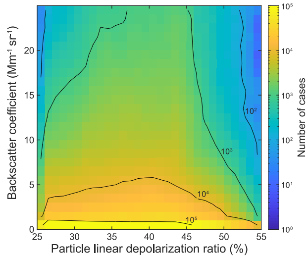
Figure B2. 2d histogram MS:s of rev2: particle backscatter coefficient ( \beta ) and rev2: particle linear depolarization ratio ( \delta ) for the WALES cirrus observations during CIRRUS-HL.
