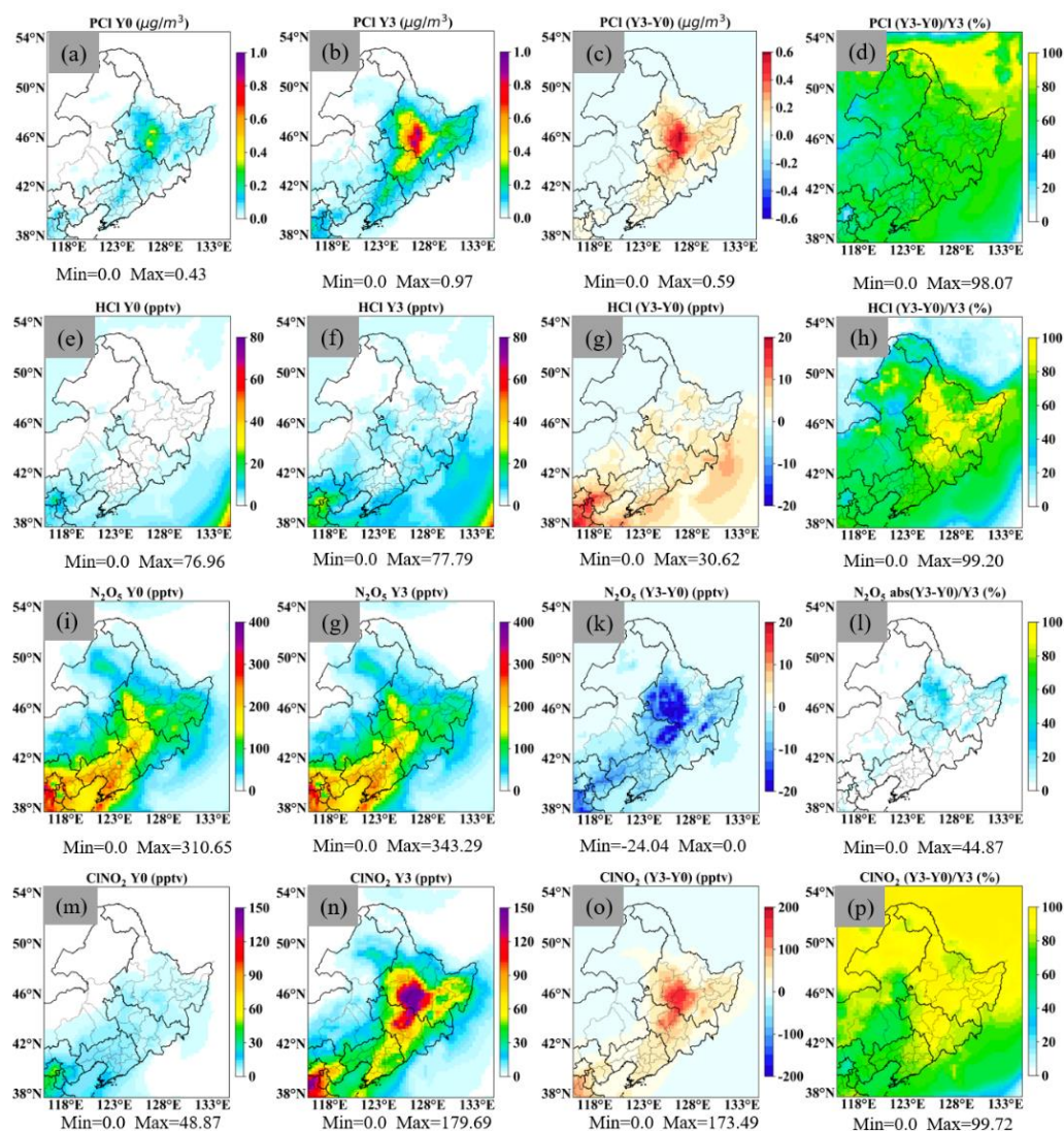
Figure 4 The spatial distribution of the impact of chlorine emissions and chlorine chemical reactions on pollutants (PCl, HCl, \text{N}_2\text{O}_5 , and \text{ClNO}_2 ).
