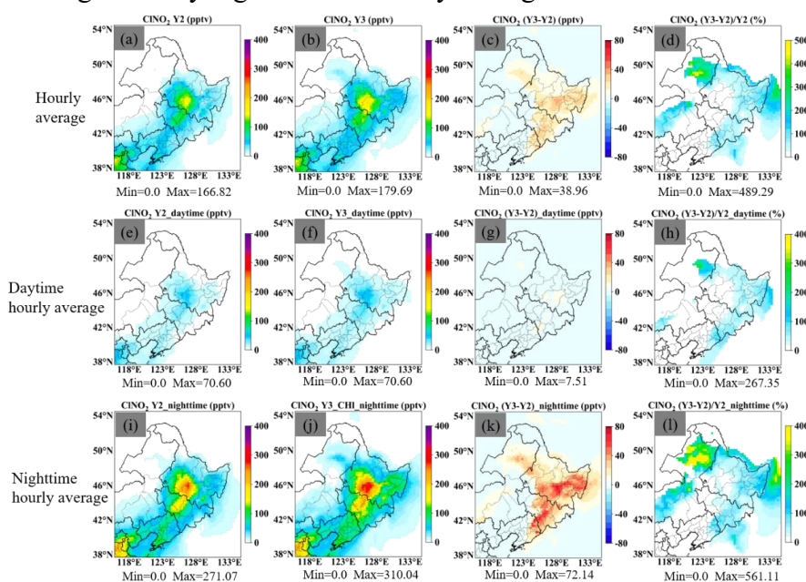
Figure 6 The quantitative contribution of ground surface chemistry to hourly
