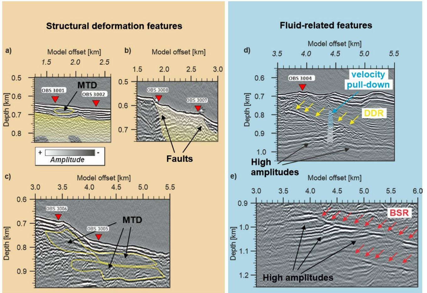
Figure 10: Enlarged seismic sections highlighting key structural and fluid-related features within profiles A and B. Left panel: Structural deformation features showing a) mass-transport deposits (MTDs) and chaotic seismic facies (CSF, yellow semi-transparent zone) from profile A; b) faults and CSF together with observed gas-flares (Hillman et al., 2018) on profile B; and c) MTDs along profile B. The faults are interpreted as zones of structural deformation and potential fluid pathways. Right panel: Fluid-related features exhibiting the downward-dipping reflector (DDR; yellow arrows), the seismic chimney (SC, semi-transparent light blue area), and associated high-amplitude reflections beneath the DDR in profile A. The SC is marked by a velocity pull-down in the upper part of the seismic anomaly. e) displays the bottom-simulating reflectors (BSRs; red arrows) and underlying high-amplitude anomalies in profile B. The high-amplitude reflections are interpreted as indicators for free gas accumulation. Boxes in figures 8 and 9 indicate the location of the enlarged sections shown here.
