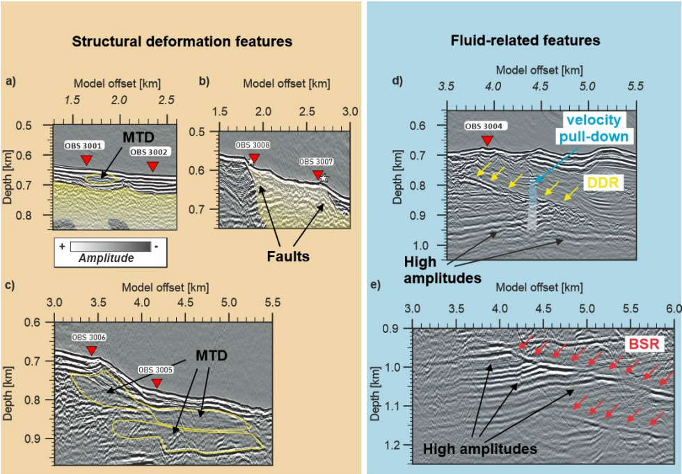
Figure 10: Enlarged seismic sections highlighting key structural and fluid-related features within profiles A and B. Left panel: Structural deformation features showing a) mass-transport deposits (MTDs) and chaotic seismic facies (CSF, yellow semi-transparent zone) from profile A; b) faults and CSF together with observed gas-flares (Hillman et al., 2018) on profile B; and c) MTDs along profile B. The faults are interpreted as zones of structural deformation and potential fluid pathways. Right panel: Fluid-related features exhibiting the downward-dipping reflector (DDR; yellow arrows), the seismic chimney (SC, semi-transparent light blue area), and associated high-amplitude reflections beneath the DDR in profile A. The SC is marked by a velocity pull-down in the upper part of the seismic anomaly. e) displays the bottom-simulating reflectors (BSRs; red arrows) and underlying high-amplitude anomalies in profile B. The high-amplitude reflections are interpreted as indicators for free gas accumulation. Boxes in figures 8 and 9 indicate the location of the enlarged sections shown here.
