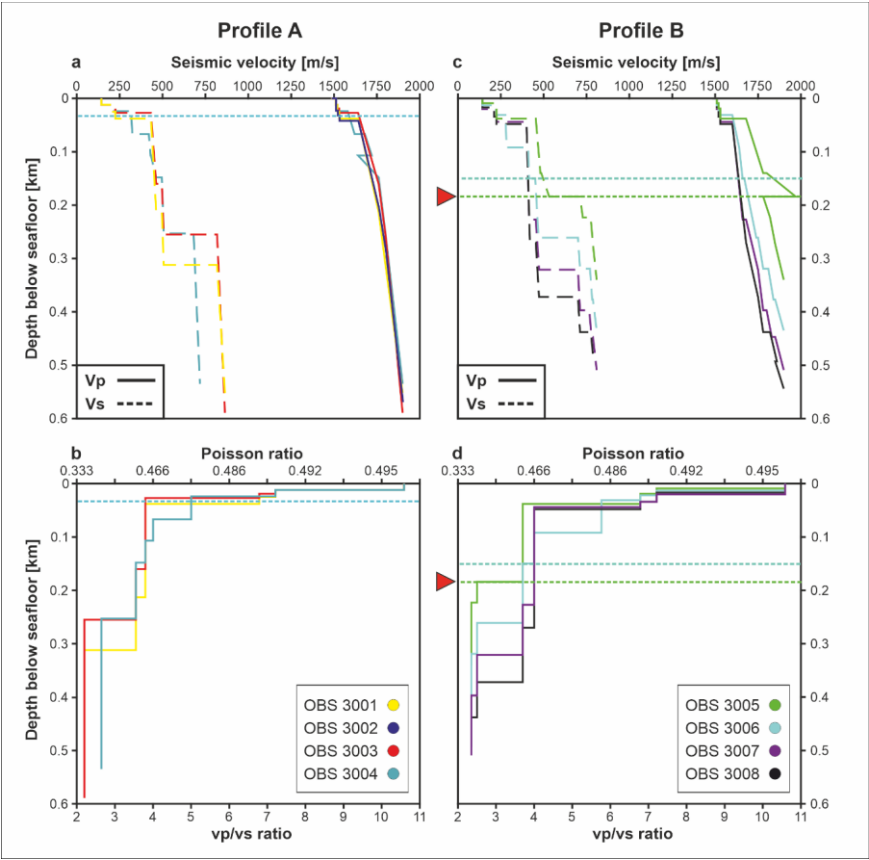
Fig. 76: 1-D velocity and ratio profiles for OBS stations along profiles A and B. (a) 1-D P-wave (solid lines) and S-wave (dashed lines) velocity profiles for OBSs 3001-3004 along profile A. (b) Corresponding 1-D Vp/Vs and Poisson's ratios. Note: Poisson's ratio is non-linearly related to the Vp/Vs-ratio. (c) 1-D P-wave (solid lines) and S-wave (dashed lines) velocity profiles for OBSs 3005-3008 along profile B. (d) Corresponding 1-D Vp/Vs and Poisson's ratios. The horizontally dashed lines represent the theoretical base of the GHSZ (after Badhani, 2016) and the red triangle marks the observed BSR depth at OBS 3005. The different depth of the theoretical GHSZ are a direct response to the prevailing pressure and temperature conditions in the shallow setting.
