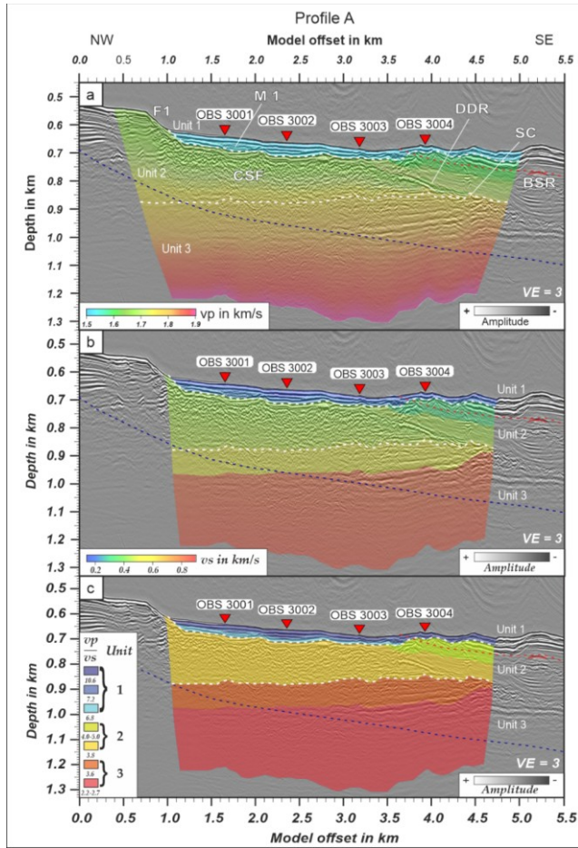
Fig. 65: Seismic velocity structure models of profile A. (a) P-wave velocity, (b) S-wave velocity, and the corresponding (c) Vp/Vs-ratio models overlaying the 2-D MCS seismic data. The seismic section is vertically exaggerated by a factor of three. Inverted red triangles indicate the position of the OBSs along the profile. Seismic anomalies are pointed out: BSR – bottom-simulating reflector, CSF – chaotic seismic facies, DDR – downward dipping reflector, F1 – fault, M1 – mass transport deposits (MTD), and SC – seismic chimney structure. The dashed white lines mark the boundaries of Unit 2. The dotted red line marks the theoretical base of the present-day GHSZ, calculated using a bottom-water temperature of 9° C and a geothermal gradient of 22 °C/km. The blue dotted line indicates the estimated GHSZ base during the Last Glacial Maximum (LGM), assuming a bottom temperature of 4 °C and the same thermal gradient (both after Badhani, 2016). Note: The theoretical BSR marks the upper limit of the GHSZ. At this shallow depth, conditions are not fully stable, so the BSR does not precisely follow the seafloor.
