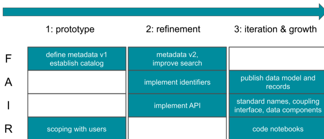
25 Figure 2: Schematic diagram showing the three phases on the path to FAIR models, along with specific steps related to the principles Findable (F), Accessible (A), Interoperable (I), and Resuable (R). In phases 1 and 2, metadata v1 and metadata v2 refer to metadata about the models (e.g., Supplement Tables 2 and 3). In phase 3, the data model and records refer to the data model and records for the catalog items (e.g., Serna et al., 2025). API: Application Programming Interface.
