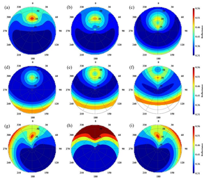
Figure 7: Angular distribution of canopy reflectance in the NIR band: (a-f) for an aspect of 0^\circ and slopes of 0^\circ , 10^\circ , 20^\circ , 30^\circ , 40^\circ , and 50^\circ ; (g-i) for a slope of 20^\circ and aspects of 90^\circ , 180^\circ , and 270^\circ .
