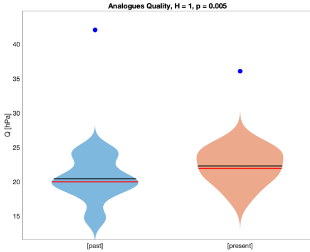
Figure 4. Analogue quality scores TS14 ( Q ) for the set of analogues selected dates in the past (1950–1986, blue) and present (1987–2024, orange) periods. Violin plots show the distribution of mean Euclidean distances between 42 analogue SST patterns and randomly selected JJAS days from the same period. The horizontal red and black lines indicate the mean and median of each distribution, respectively. The filled blue dots mark the actual Q values computed between the target 2025 SST event and its selected analogues. A lower Q indicates a better match. The statistical difference between past and present distributions is confirmed by a two-tailed Cramér–von Mises test ( p = 0.005 ).
