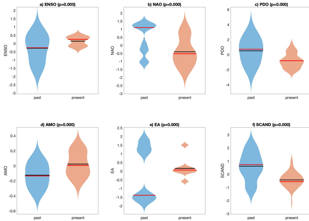
283 Figure 3. Violin plots comparing the distributions of natural variability indices during analogue dates in the 284 past (1950–1986, blue) and present (1987–2024, orange) periods. The indices include: a) El Niño–Southern 285 Oscillation (ENSO), b) North Atlantic Oscillation (NAO), c) Pacific Decadal Oscillation (PDO), d) Atlantic 286 Multidecadal Oscillation (AMO), e) East Atlantic pattern (EA), and f) Scandinavian pattern (SCAND). Each 287 violin shows the full probability density of the distribution, with horizontal red and black lines indicating the 288 mean and median, respectively. The width of the violin reflects the relative frequency of values. All 289 comparisons yield statistically significant differences between past and present periods (two-tailed Cramér– 290 von Mises test, p < 0.001 ), suggesting that the underlying state of large-scale climate modes has shifted over 291 time.
