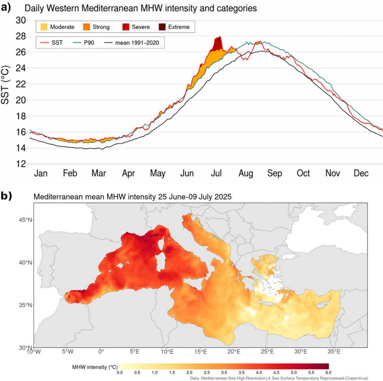
178 Figure 1. a) Daily SST averaged over the Western Mediterranean Sea for 2025 (red), together with the 179 1991–2020 daily climatological mean (black line) and the 90th percentile MHW threshold (P90, teal 180 line). Shading indicates the MHW category (moderate, strong, severe, extreme) following Hobday et 181 al. (2016, 2018). b) Mean MHW intensity (temperature anomaly above the 1991–2020 climatology, in °C)
