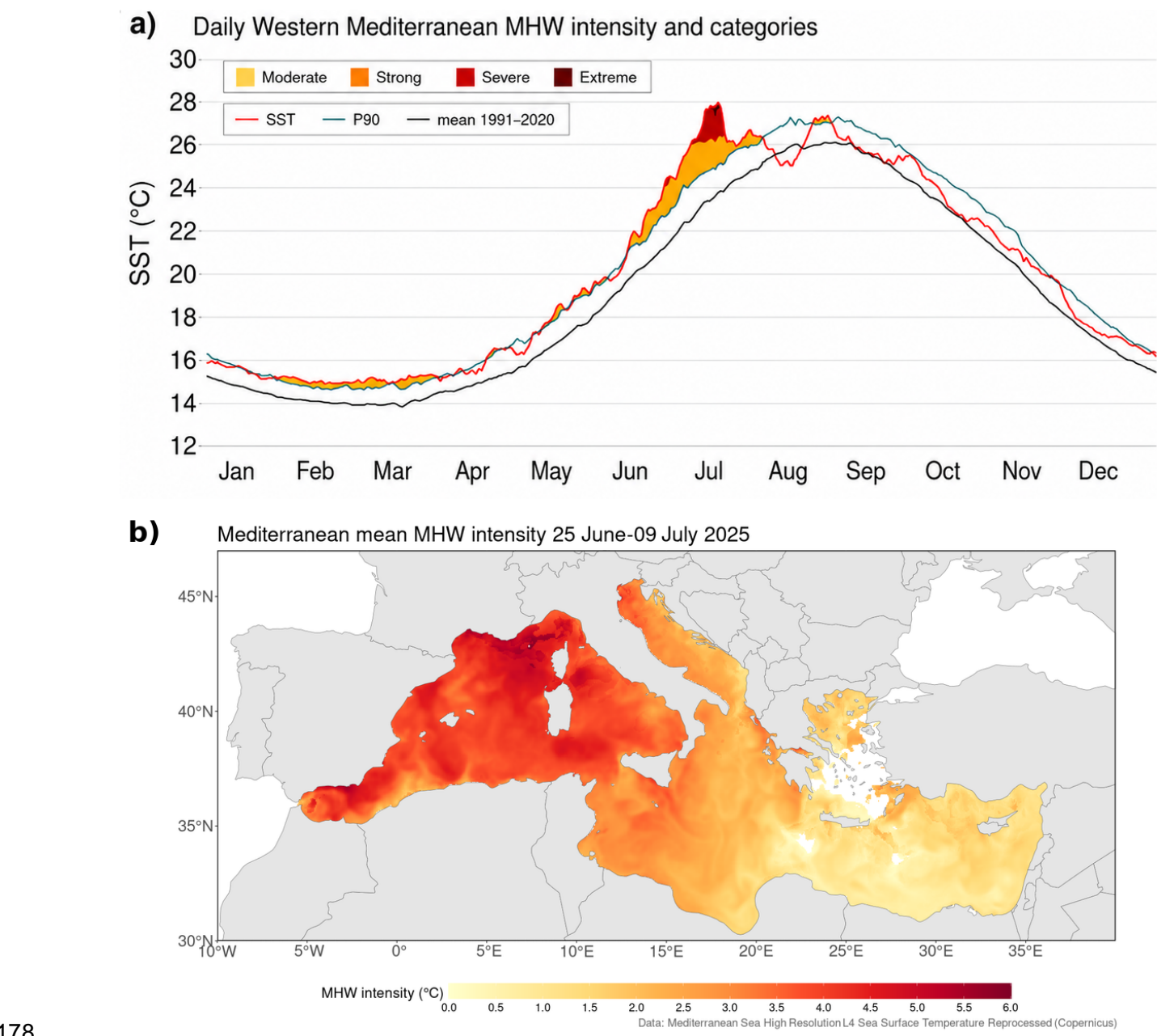
178 179 Figure 1. a) Daily SST averaged over the Western Mediterranean Sea for 2025 (red), together with the 180 1991–2020 daily climatological mean (black line) and the 90th percentile MHW threshold (P90, teal
