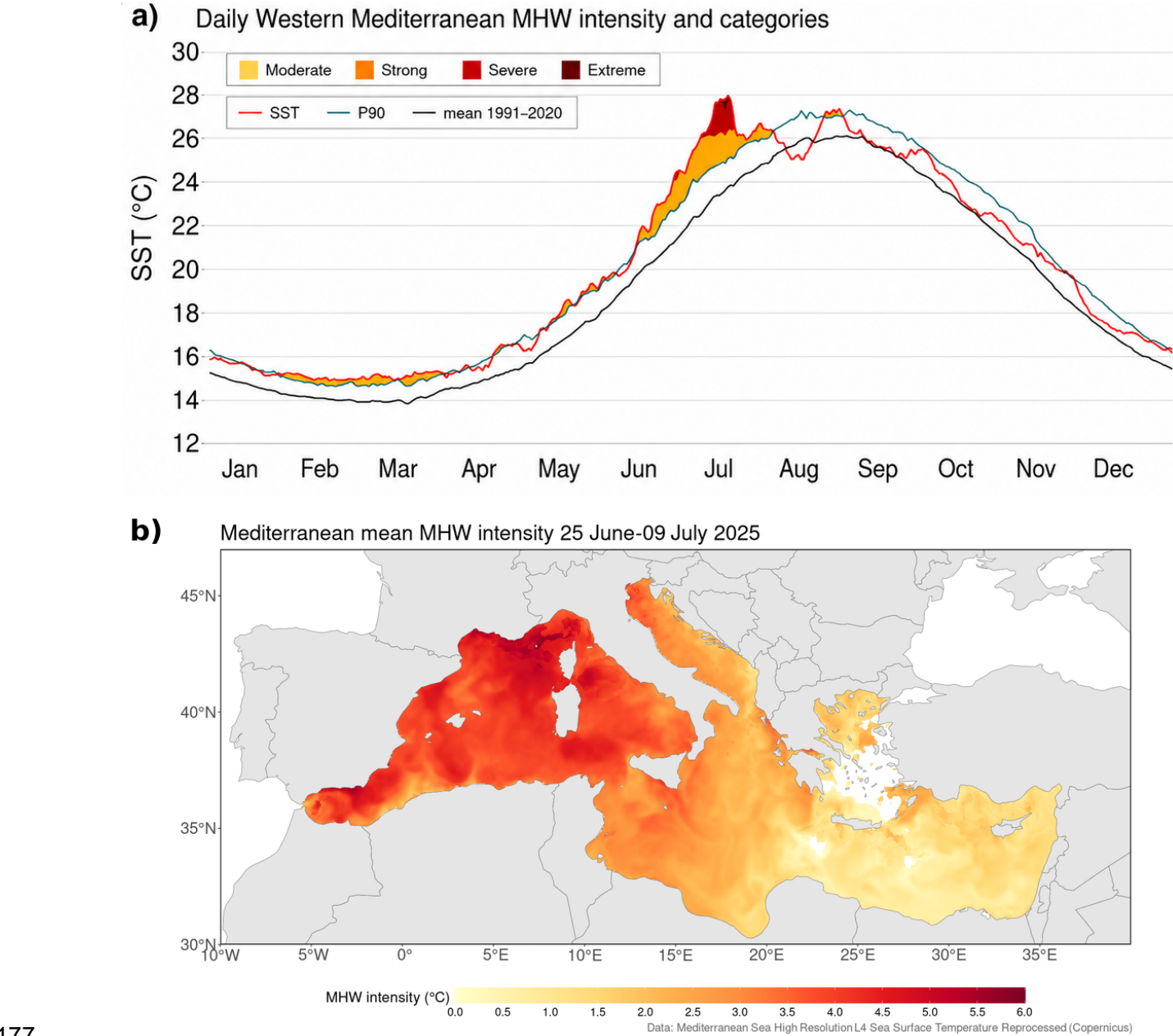
Figure 1. a) Daily SST averaged over the Western Mediterranean Sea for 2025 (red), together with the 1991–2020 daily climatological mean (black line) and the 90th percentile MHW threshold (P90, teal line). Shading indicates the MHW category (moderate, strong, severe, extreme) following Hobday et al. (2016, 2018). b) Mean MHW intensity (temperature anomaly above the 1991–2020 climatology, in °C)
