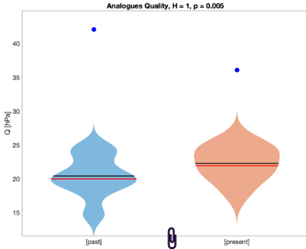
Figure 4. Analogue quality scores (TS14) ( Q ) for the set of analogues selected dates in the past (1950–1986, blue) and present (1987–2024, orange) periods. Violin plots show the distribution of mean Euclidean distances between 42 analogue SST patterns and randomly selected JJAS days from the same period. The horizontal red and black lines indicate the mean and median of each distribution, respectively. The filled blue dots mark the actual Q values computed between the target 2025 SST event and its selected analogues. A lower Q indicates a better match. The statistical difference between past and present distributions is confirmed by a two-tailed Cramér–von Mises test ( p = 0.005 ).
