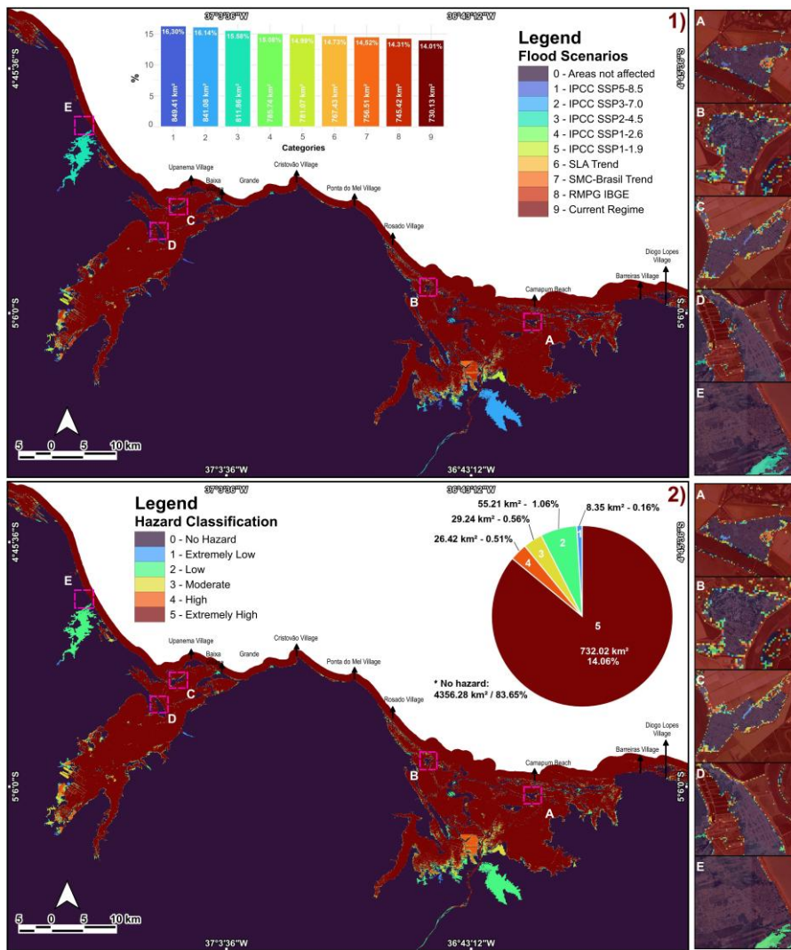
Figure 9: Classification of MSLR scenarios in the study area (1) and classification of tidal flooding hazards (2) by sector. The far-right column shows the scale zones in the cities of the study area. The graphs on the maps indicate the percentages of the total area occupied. Map uses the base map data from Bing Maps (© Microsoft).
