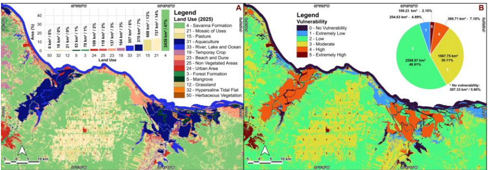
Figure 11: Land use in the study area (A) and vulnerability classification (B). The graphs at the top show the percentages of the areas occupied by each class in ascending order. The graphs at the top indicate the percentages of areas occupied by each class. Map A using data from Mabpiomas (2025).
