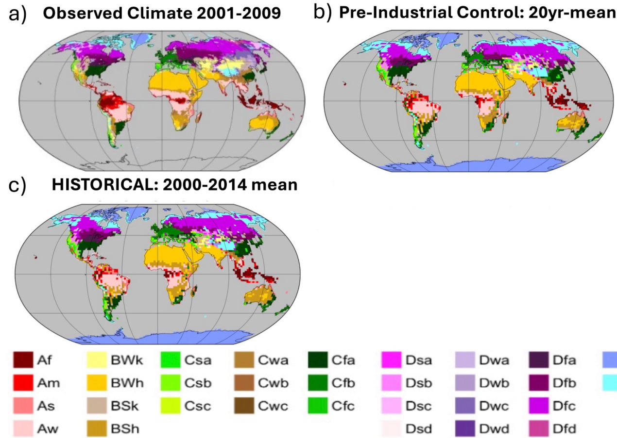
Figure 9. Köppen-Geiger climate classifications of a) observed 2001-2009 climatology (ERA5), b) the pre-industrial and c) historical runs. Colorscheme is from Kottek et al. (2006). Observed climate from ERA5 at 0.5°x0.5° resolution.
