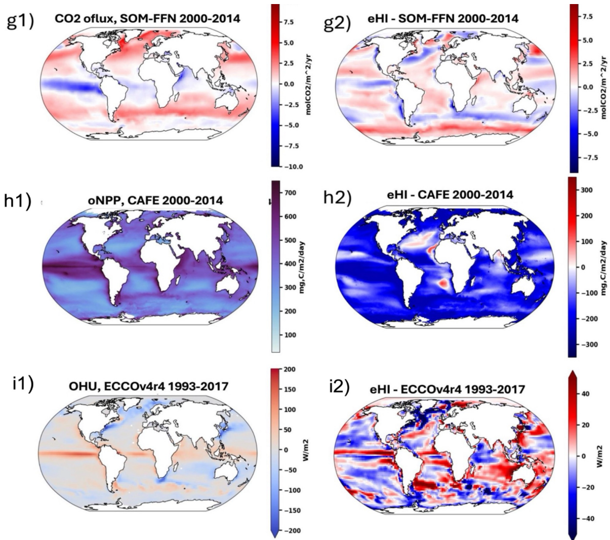
Figure 5. Observational and observation-based estimates and model spatial biases averaged over the period of the observations. a1) Atmospheric CO 2 concentration anomalies from the global mean from Carbon Tracker averaged over 2000-2014. a2) Atmospheric CO 2 concentration anomalies, model biases from Carbon Tracker, b1) GISTEMP average 2000-2014, b2) Surface air temperature model biases from GISTEMP v4 (anomalies from 1951-1980) averaged over 2000-2014, c1) Precipitation average 2001-2010 from GPCPv4, c2) historical precipitation biases over land fro GPCPv4, d1) Land carbon flux taken from Carbon Tracker between 2000-2014, d2) land
