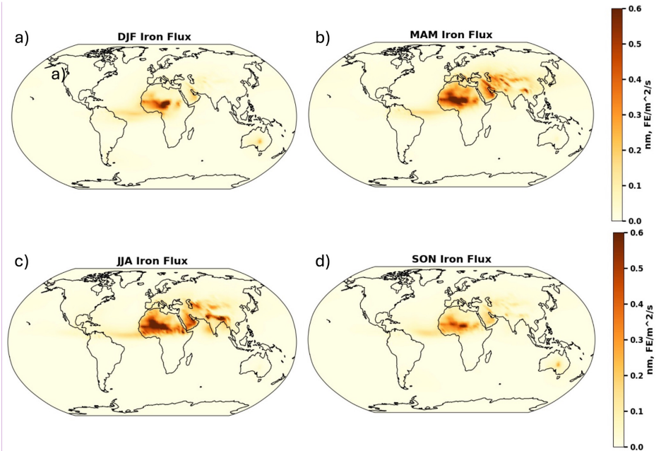
Figure 6. Seasonal averages of dust iron flux deposited at the surface of the ocean (nm, Fe/m 2 /s).
