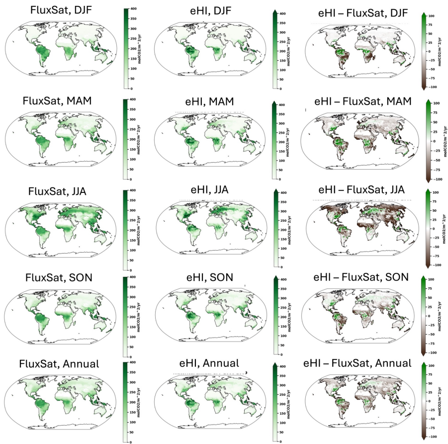
Figure SUPP3: Land carbon seasonality from eHI and FluxSat.
