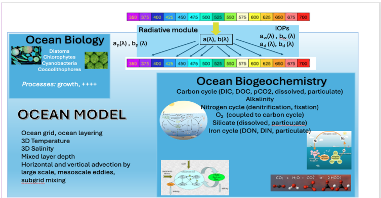
103 104 Figure 3. Schematic diagram of the NOBM in GISS ModelE2.1-CC2
