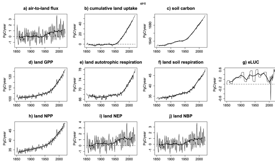
Figure SUPP2: Land fluxes and soil carbon from eHI, with annual (thin line), 20-year moving average (thick line), and zero line (dashed line). a) air-to-land flux, b) cumulative land uptake since 1850, c) soil carbon stocks, d) land gross primary productivity (GPP), e) land autotrophic respiration, f) land soil respiration, g) emissions due to land use change (LUC), h) land net primary productivity (NPP), i) land net ecosystem productivity (NEP), and j) land net biome productivity (NBP).
