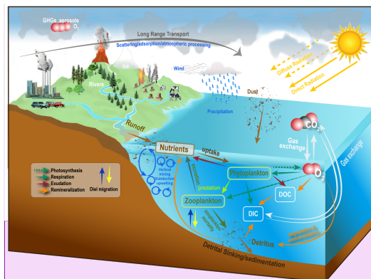
Figure 2. Schematic diagram of the ocean carbon cycle model (NOBMg). credit: Jay Friedlander, NASA-GSFC.
