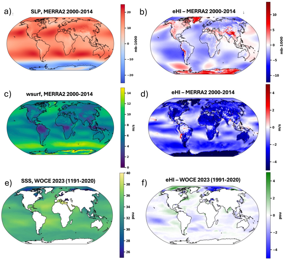
41 42 Figure SUPP1: SLP, wsurf and SSS from eHI and observations 43 44
