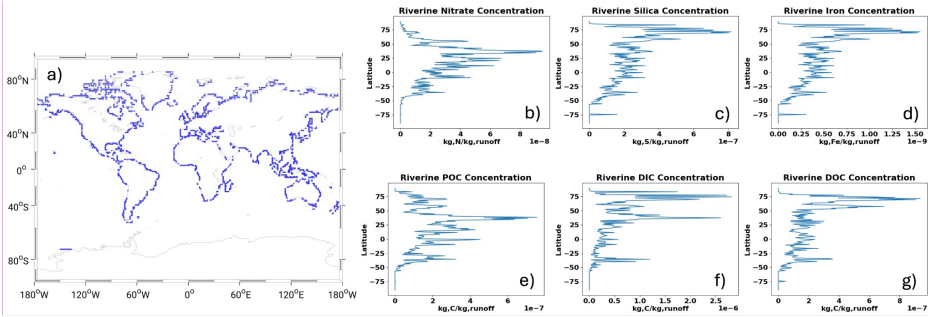
Figure 8. a) Sites of continental runoff release in ModelE. b) Zonally averaged concentrations of nitrate, silica, dissolved iron, POC, DIC and DOC.
