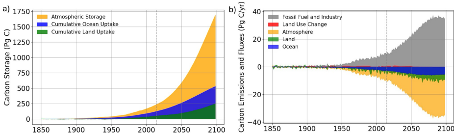
Figure 25. a) Combined emissions driven historical and SSP5-8.5 yearly global mean trajectories of cumulative land and ocean carbon uptake and atmospheric carbon storage. The gray dashed line corresponds to the year 2014. b) Components of the carbon budget in terms of CO 2 flux from the emission driven historical and SSP5-8.5 experiments. Positive flux is defined as CO 2 emitted from fossil fuel/industry and land use change, and negative flux is defined as partitioning of CO 2 into the atmosphere, land, and ocean reservoirs. The land component excludes land use change. Left and right of the gray dashed line correspond to the historical and future periods, respectively.
