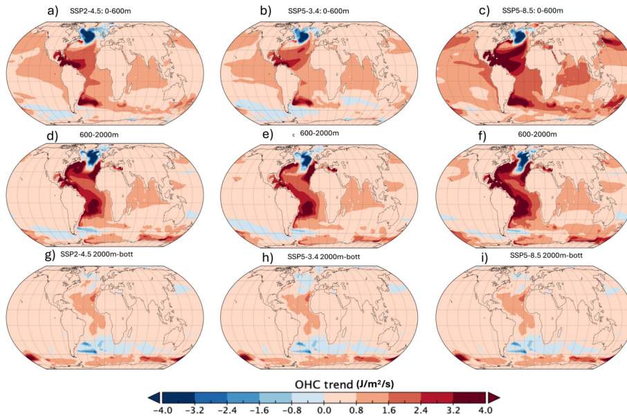
65 66 Figure 20. Ocean heat content trend ( \text{J/m}^2/\text{s} ) in GISS2.1-CC2 from three different SSP scenarios, vertically integrated: a, 67 b,c) from surface to 600m, d,e,f) 600-2000m, g,h,i) 2000m-bottom. Left column is for SSP2-4.5, middle column for SSP5- 68 3.4, and the right column for SSP5-8.5.
