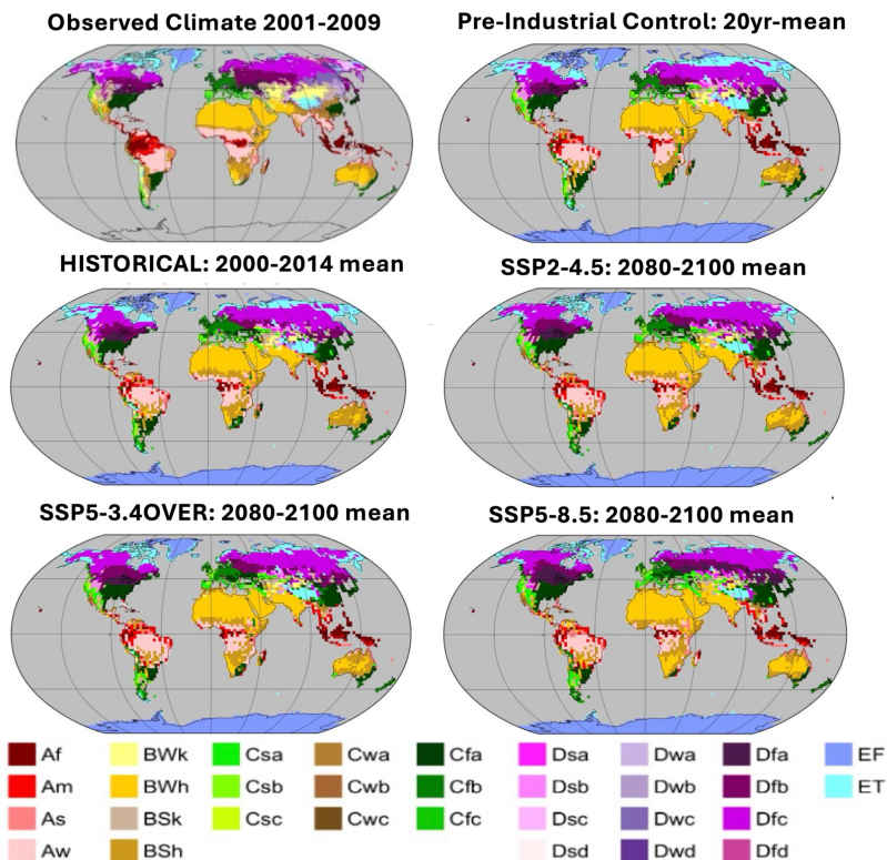
Figure 26. Köppen-Geiger climate classifications of observed 2001-2009 climatology (ERA5) and the 5 runs. Colorscheme is from Kottek et al. (2006). Observed climate from ERA5 at 0.5°x0.5° resolution.
