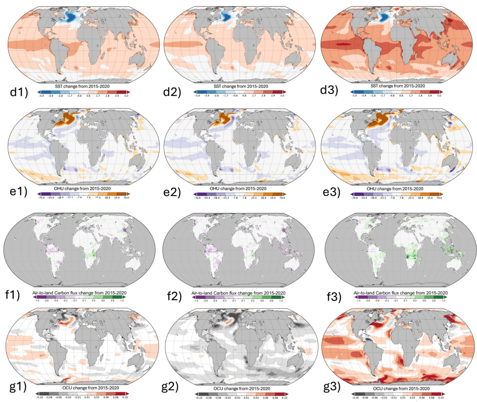
Figure 17. Response to future forcing: changes in SSP2-4.5 (left column), SSP3-3.4 (middle column), SSP5-8.5 (right column). Shown are differences of averaged fields over the last 20 years (2080-2100) from late historical (2015-2020). a1,2,3) surface air temperature (°C), b1,2,3) precipitation (mm/day), c1,2,3) soil liquid water change (kg/m²), d1,2,3) sea surface temperature (°C), e1,2,3) ocean heat uptake (W/m²), f1,2,3) air-to-land carbon flux (gC/m²/day), g1,2,3) air-to-sea carbon flux (gC/m²/day).
