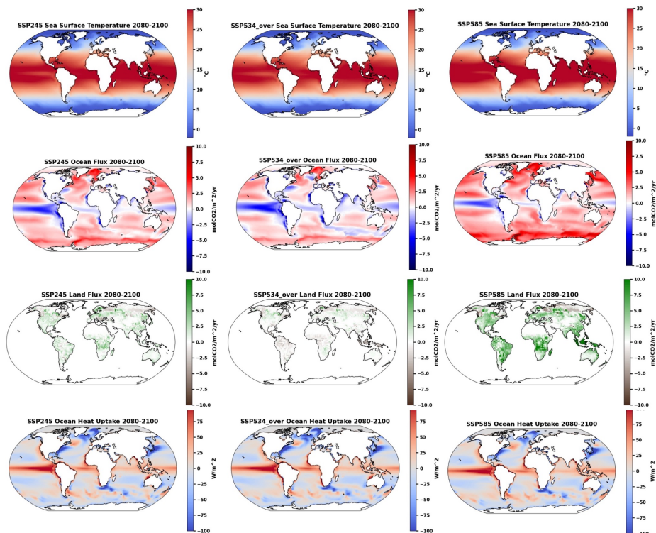
Figure SUPP4: Averaged climatologies of the last 20 years in SSPs.
