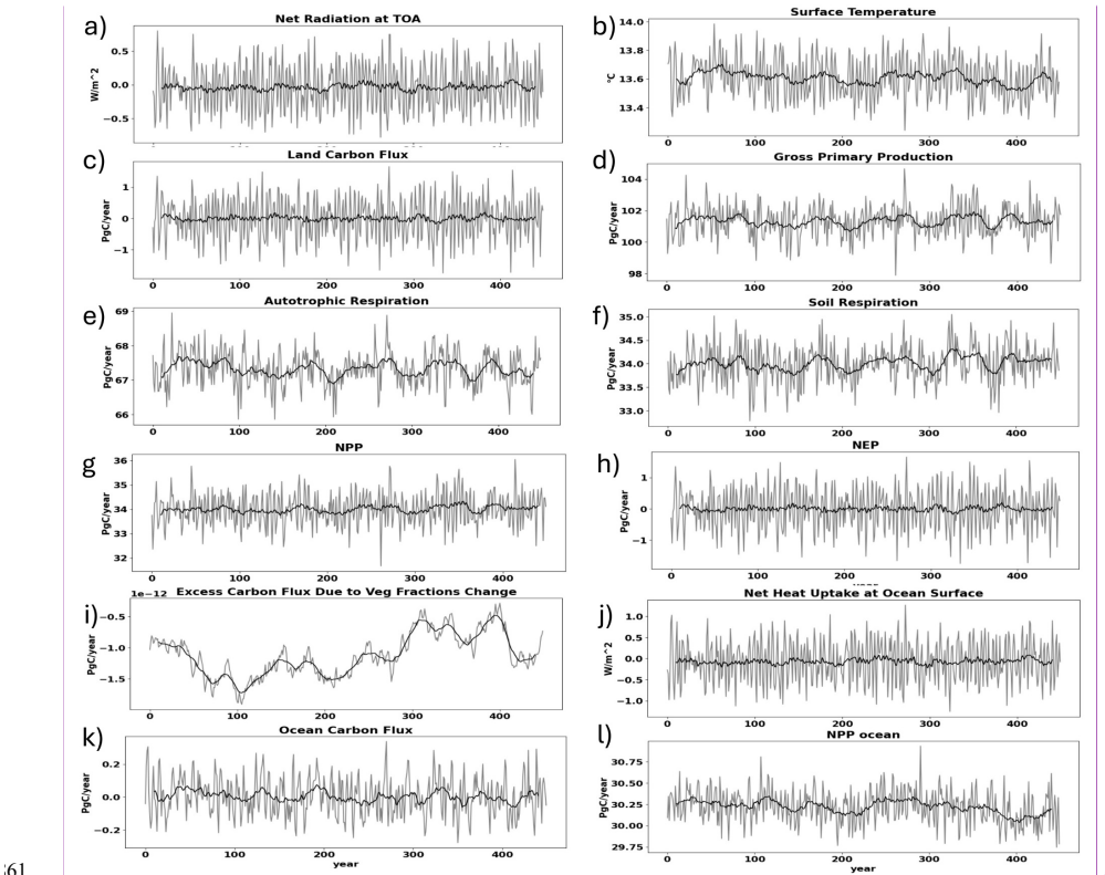
61 62 Figure 10. Temporal evolution of preindustrial control fields: a) net radiation at top of the atmosphere (TOA), b) surface air temperature, 63 c) land carbon flux, d) gross primary production (GPP), e) autotrophic respiration, f) soil respiration, g) net primary production on land 64 (NPP = GPP - autotrophic respiration) h) net ecosystem production (NEP = NPP - soil respiration), i) excess carbon flux due to vegetation 65 fractions change, j) net heat uptake by ocean, k) ocean air-sea carbon flux, l) net ocean primary production (NPP ocean). Annual mean 66 fields are shown in gray. 20yr averages are shown in black. The horizontal axis is in years from the PI control run. Units are shown on 67 the vertical axes. All fluxes are positive down into the surface (land or ocean).
