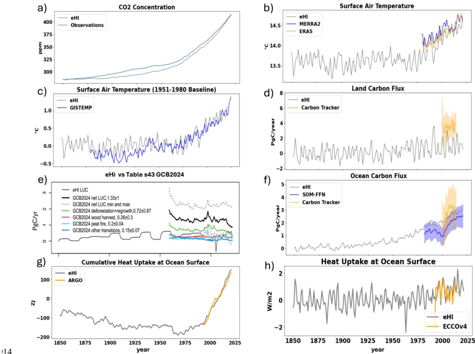
14 15 Figure 12. Annual Time series of a) atmospheric CO2 concentration from the model (eHI) and observations from 16 input4mips (Meinshausen et al., 2017) from 1850 to 2015, and from the NOAA Global Monitoring Laboratory from 2015 17 to 2021 (Lan et al., 2022a,b), b) surface air temperature (annual mean timeseries) and superimposed estimates from 18 ERA5 and MERRA2 (see Table 3), c) change in surface air temperature from the average over the period 1951-1980 and 19 GISTEMP, d) air-to-land carbon flux from the model (eHI) compared to observations from the Carbon Tracker (shaded is 20 the uncertainty of the annual mean based on the averaging of inversions that consider different prior estimates of 21 fluxes and their uncertainties; Jacobson et al., 2023), e) components of land carbon fluxes to the atmosphere (positive is 22 flux upward) due to land use change, comparing eHI net emissions to the mean estimates of the Global Carbon Budget 23 2024 (GCB2024, Friedlingstein et al. 2025). The legend tabulates the GCB2024 means and estimated minimum and 24 maximum bounds around the mean over the period 1959-2021 where the eHI simulation and GCB2024 overlap in time,
