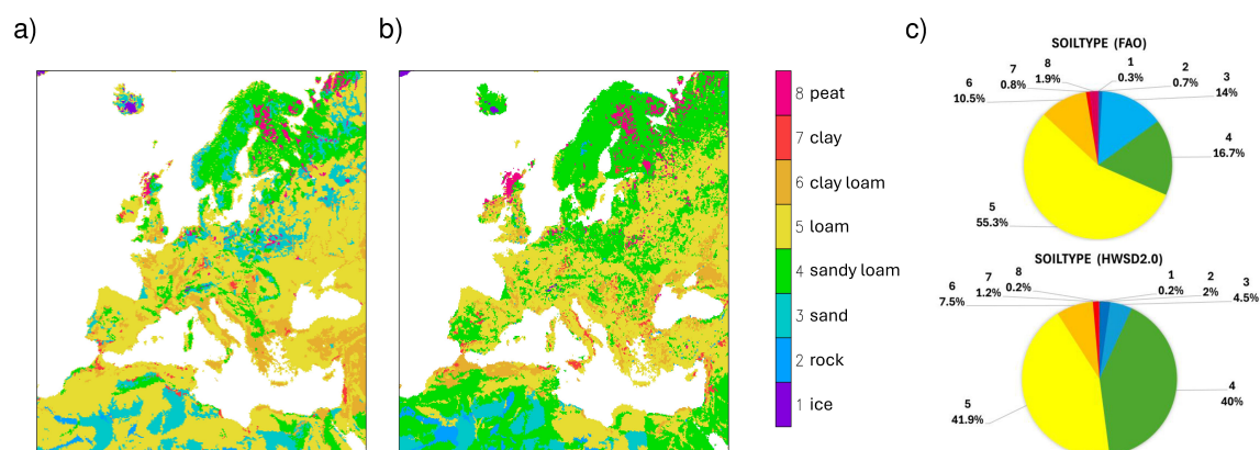
Figure 3. Default (operational) soil-type distribution based on the FAO (a) and HWSDv2 (b) datasets. The Pie chart (c) gives the portions of the spatial extent for soil types [%] shown in a and b.
