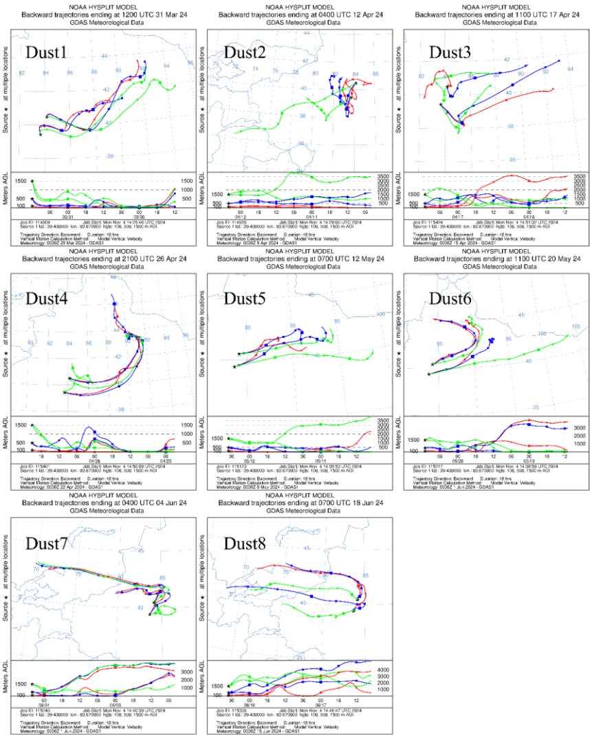
250 251 Figure 2. Backward trajectories of the eight dust-storm events.
