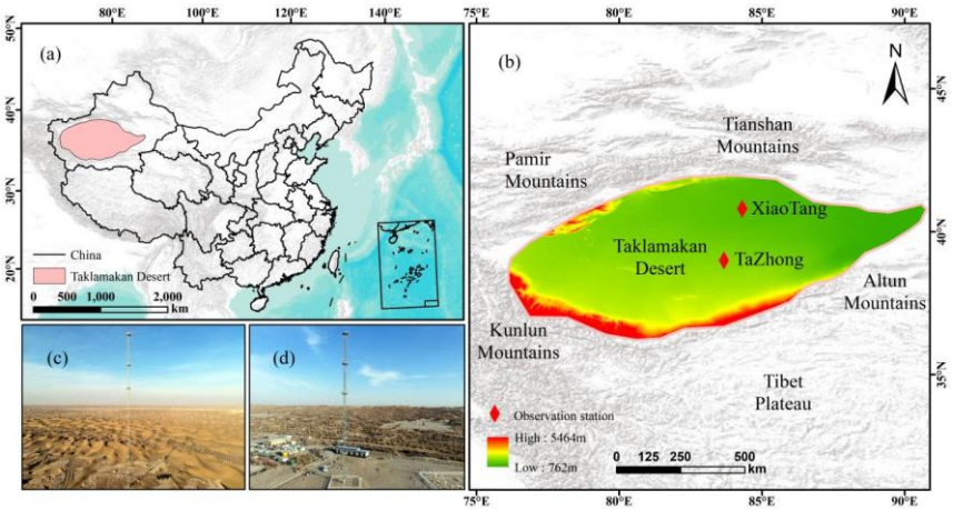
Figure 1. Location and topography of the Taklamakan Desert, including the Tazhong (TZ) and Xiaotang (XT) observation towers and site photographs. Figure 1. Location and topography of the Taklamakan Desert, showing the TZ and XT observation towers and site photographs. The base map was prepared using ArcGIS Online; attribution and copyright information follow the requirements of Esri and its data providers. Site photographs were taken by the authors.
