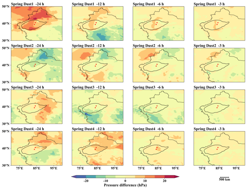
Figure 6. Sea-level pressure differences before spring dust-storm onset.
