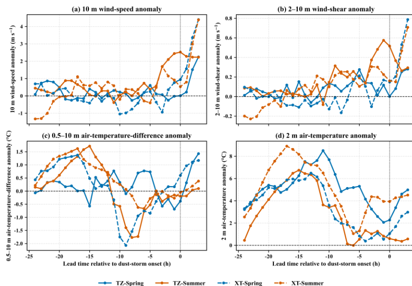
Figure 11. Composite evolution of tower-observed wind-speed, wind-shear, air-temperature-difference, and 2 m air-temperature anomalies from -24 to +3 h relative to dust-storm onset.
