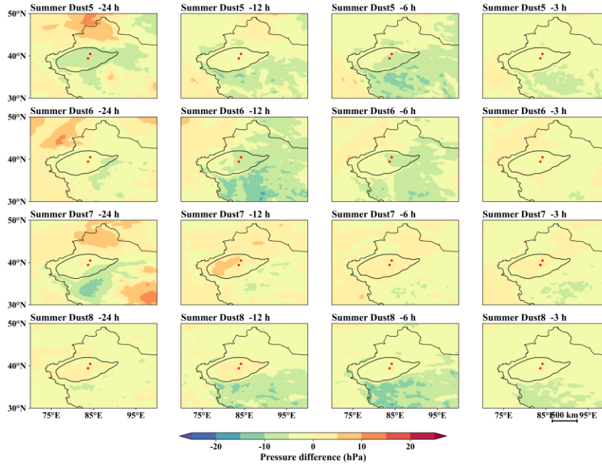
Figure 7. Sea-level pressure differences before summer dust-storm onset.
