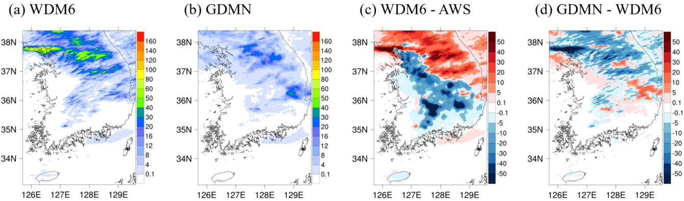
270 Figure 6: Accumulated surface precipitation (mm) during the analysis period (from 02:00 to 17:00 UTC on 6 August 2013) for (a) WDM6, (b) GDMN, and (c) the difference between WDM6 and Automatic Weather Station (AWS) observations (WDM6 minus AWS). (d) Same as (c), but for the difference between GDMN and WDM6 (GDMN minus WDM6).
